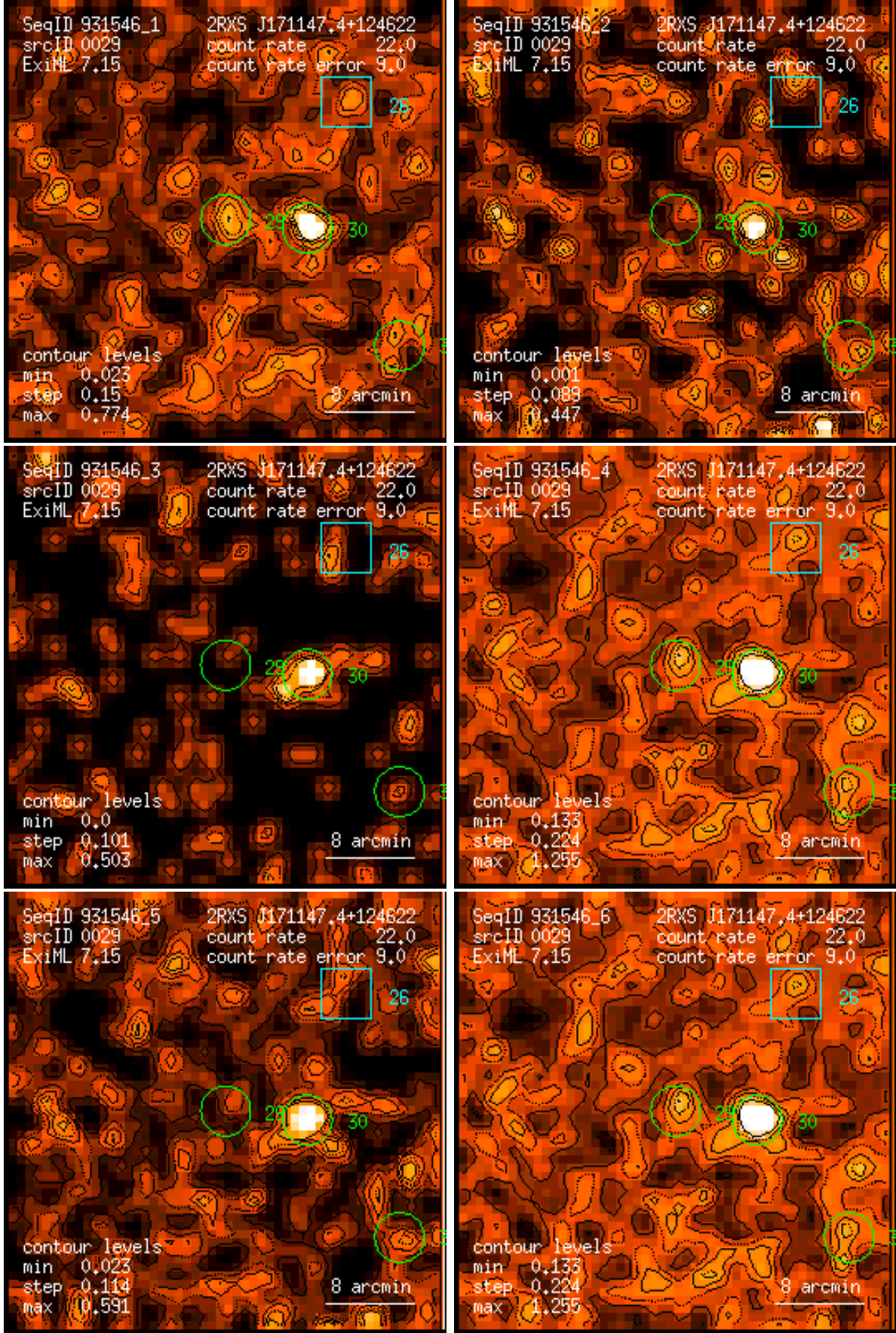
Figure 29: RASS 931546: detection 0029: band rate images, Gaussian filter: (1) PSPC channels 11 – 41, (2) 52 – 90, (3) 91 – 201, (4) 11 – 235, (5) 52 – 201, (6) 11 – 201. Broad band rates in counts/ks. Band rate contour levels in counts/ks/arcmin 2 .
