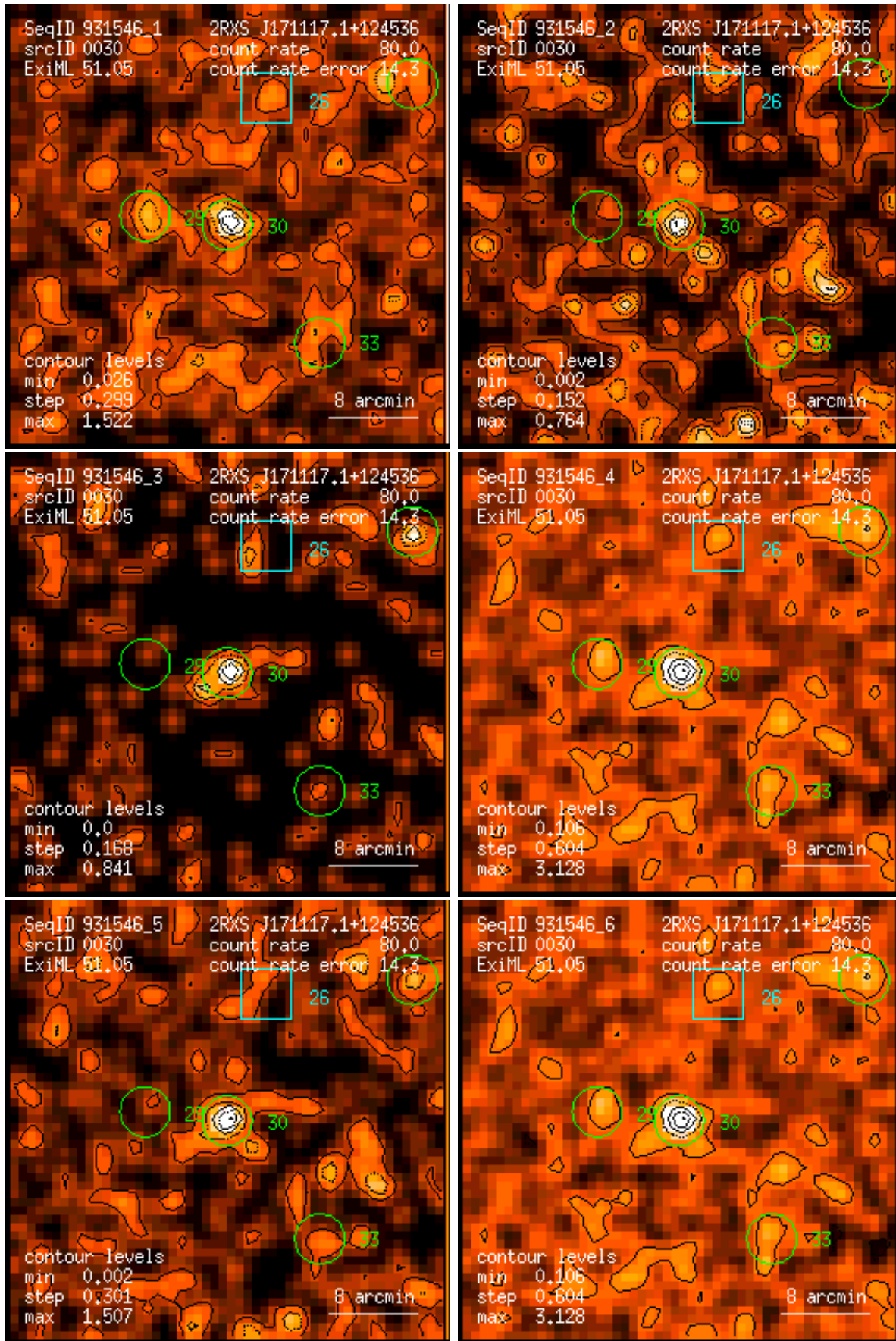
Figure 30: RASS 931546: detection 0030: band rate images, Gaussian filter: (1) PSPC channels 11 – 41, (2) 52 – 90, (3) 91 – 201, (4) 11 – 235, (5) 52 – 201, (6) 11 – 201. Broad band rates in counts/ks. Band rate contour levels in counts/ks/arcmin 2 .
