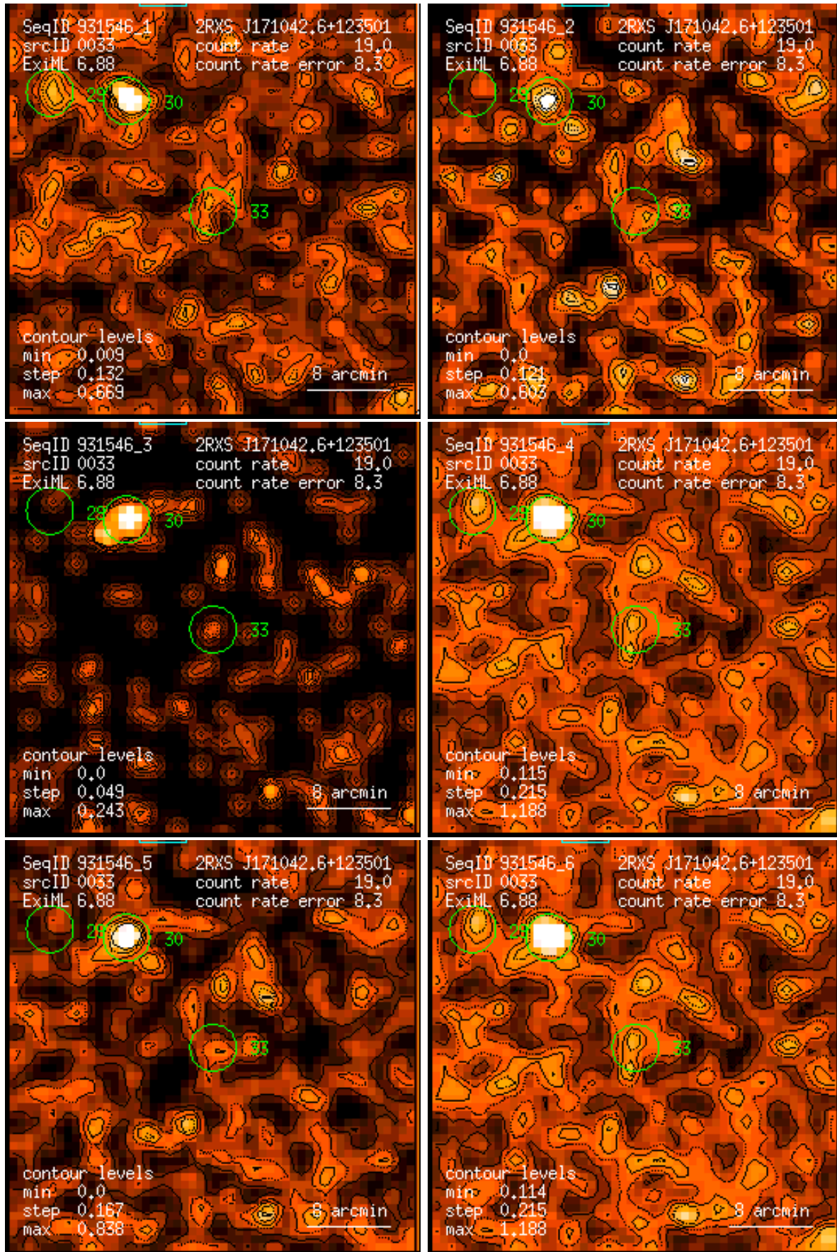
Figure 33: RASS 931546: detection 0033: band rate images, Gaussian filter: (1) PSPC channels 11 – 41, (2) 52 – 90, (3) 91 – 201, (4) 11 – 235, (5) 52 – 201, (6) 11 – 201. Broad band rates in counts/ks. Band rate contour levels in counts/ks/arcmin 2 .
