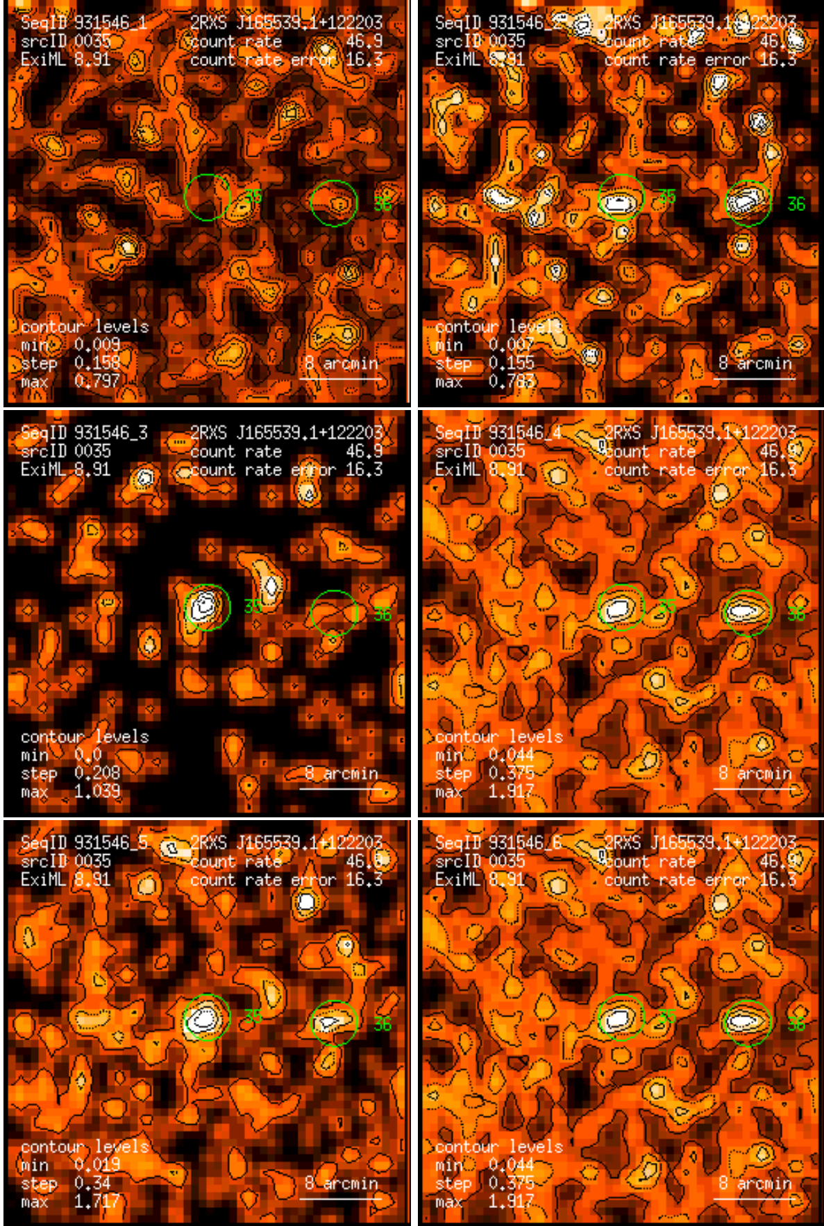
Figure 35: RASS 931546: detection 0035: band rate images, Gaussian filter: (1) PSPC channels 11 – 41, (2) 52 – 90, (3) 91 – 201, (4) 11 – 235, (5) 52 – 201, (6) 11 – 201. Broad band rates in counts/ks. Band rate contour levels in counts/ks/arcmin 2 .
