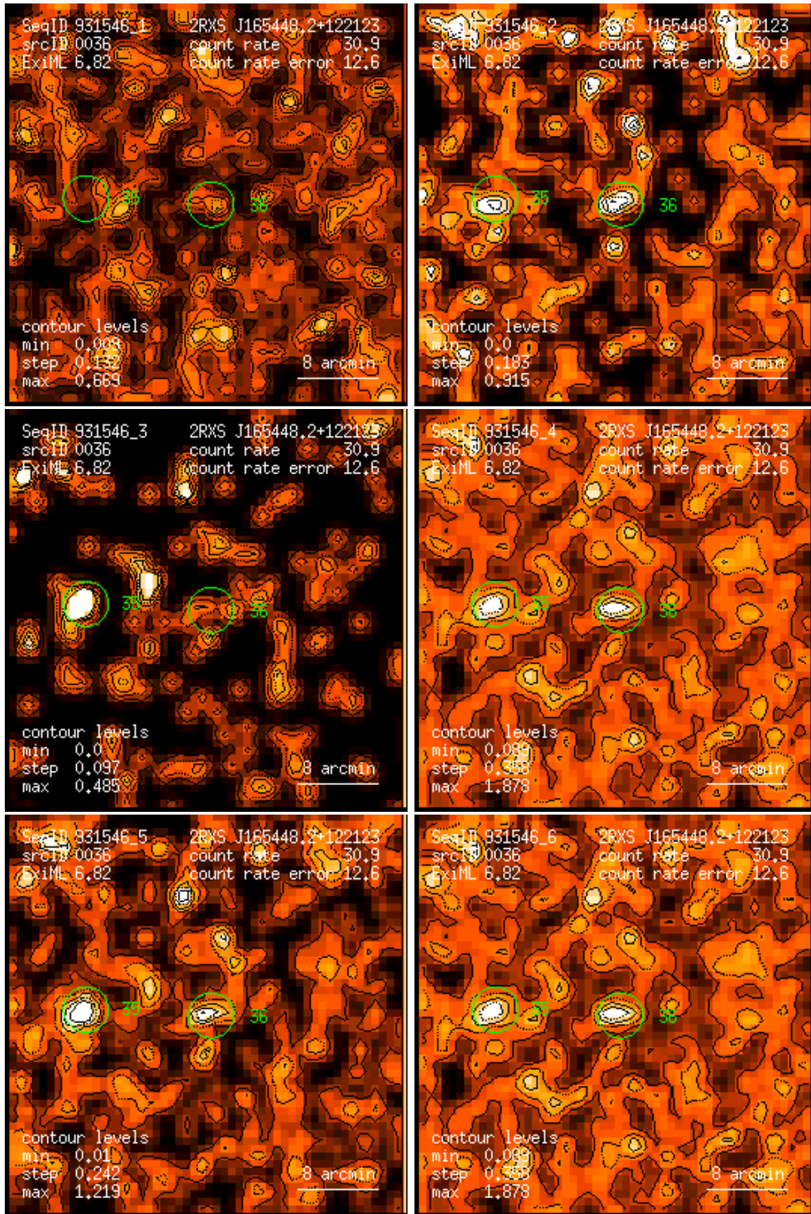
Figure 36: RASS 931546: detection 0036: band rate images, Gaussian filter: (1) PSPC channels 11 – 41, (2) 52 – 90, (3) 91 – 201, (4) 11 – 235, (5) 52 – 201, (6) 11 – 201. Broad band rates in counts/ks. Band rate contour levels in counts/ks/arcmin 2 .
