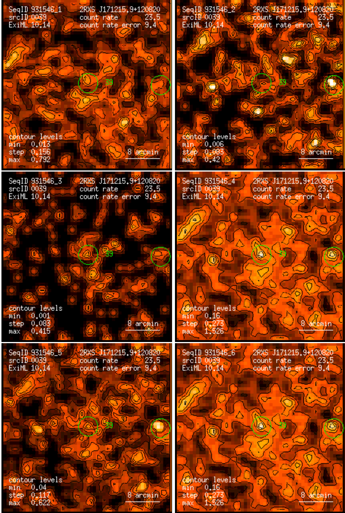
Figure 39: RASS 931546: detection 0039: band rate images, Gaussian filter: (1) PSPC channels 11 – 41, (2) 52 – 90, (3) 91 – 201, (4) 11 – 235, (5) 52 – 201, (6) 11 – 201. Broad band rates in counts/ks. Band rate contour levels in counts/ks/arcmin 2 .
