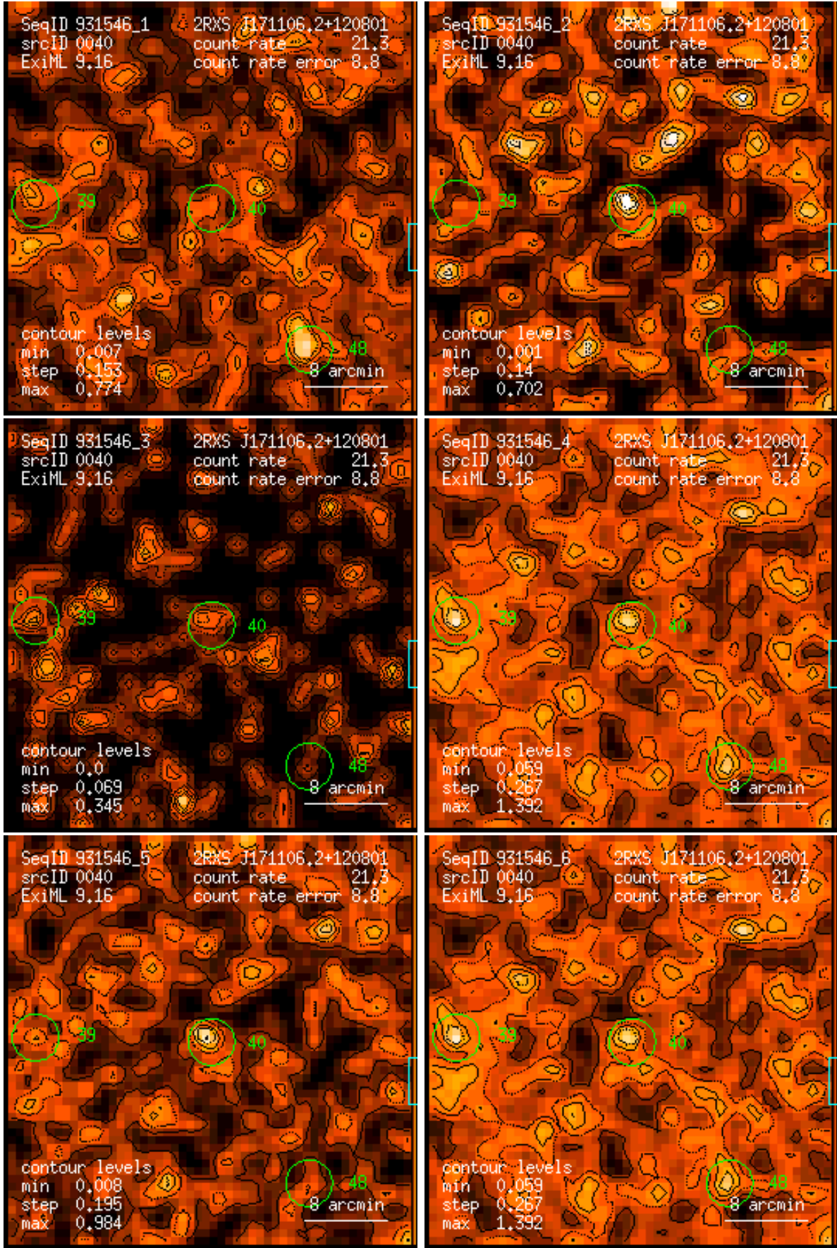
Figure 40: RASS 931546: detection 0040: band rate images, Gaussian filter: (1) PSPC channels 11 – 41, (2) 52 – 90, (3) 91 – 201, (4) 11 – 235, (5) 52 – 201, (6) 11 – 201. Broad band rates in counts/ks. Band rate contour levels in counts/ks/arcmin 2 .
