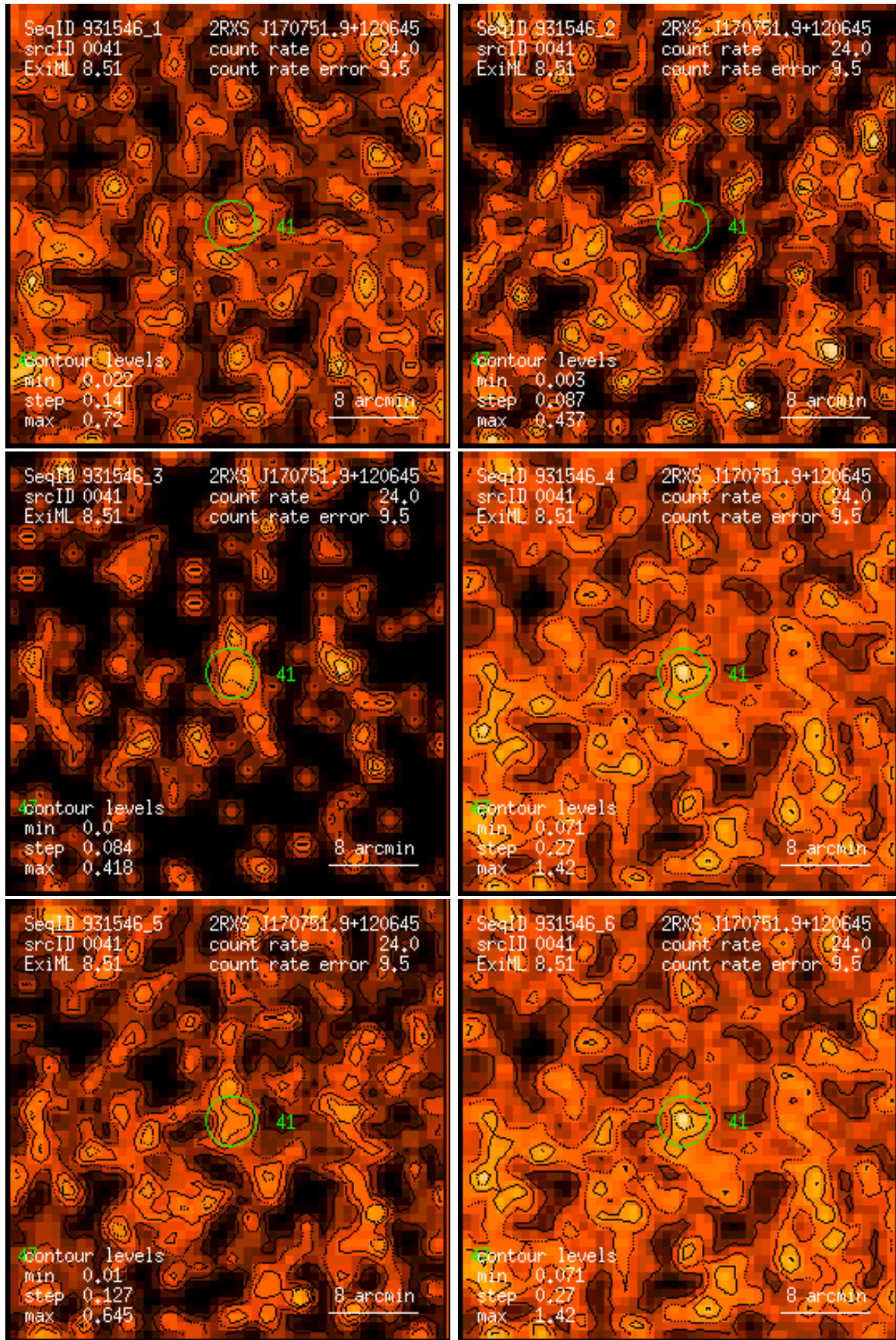
Figure 41: RASS 931546: detection 0041: band rate images, Gaussian filter: (1) PSPC channels 11 – 41, (2) 52 – 90, (3) 91 – 201, (4) 11 – 235, (5) 52 – 201, (6) 11 – 201. Broad band rates in counts/ks. Band rate contour levels in counts/ks/arcmin 2 .
