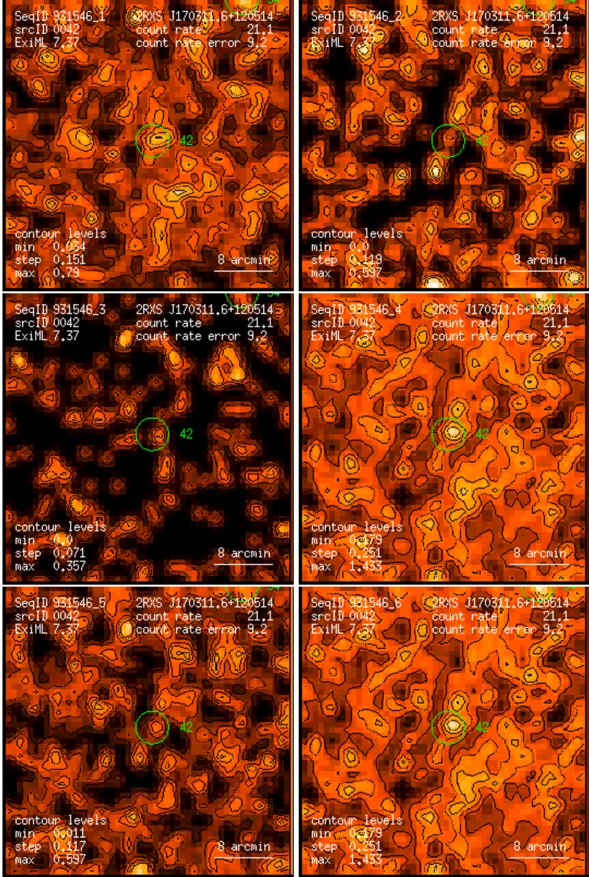
Figure 42: RASS 931546: detection 0042: band rate images, Gaussian filter: (1) PSPC channels 11 – 41, (2) 52 – 90, (3) 91 – 201, (4) 11 – 235, (5) 52 – 201, (6) 11 – 201. Broad band rates in counts/ks. Band rate contour levels in counts/ks/arcmin 2 .
