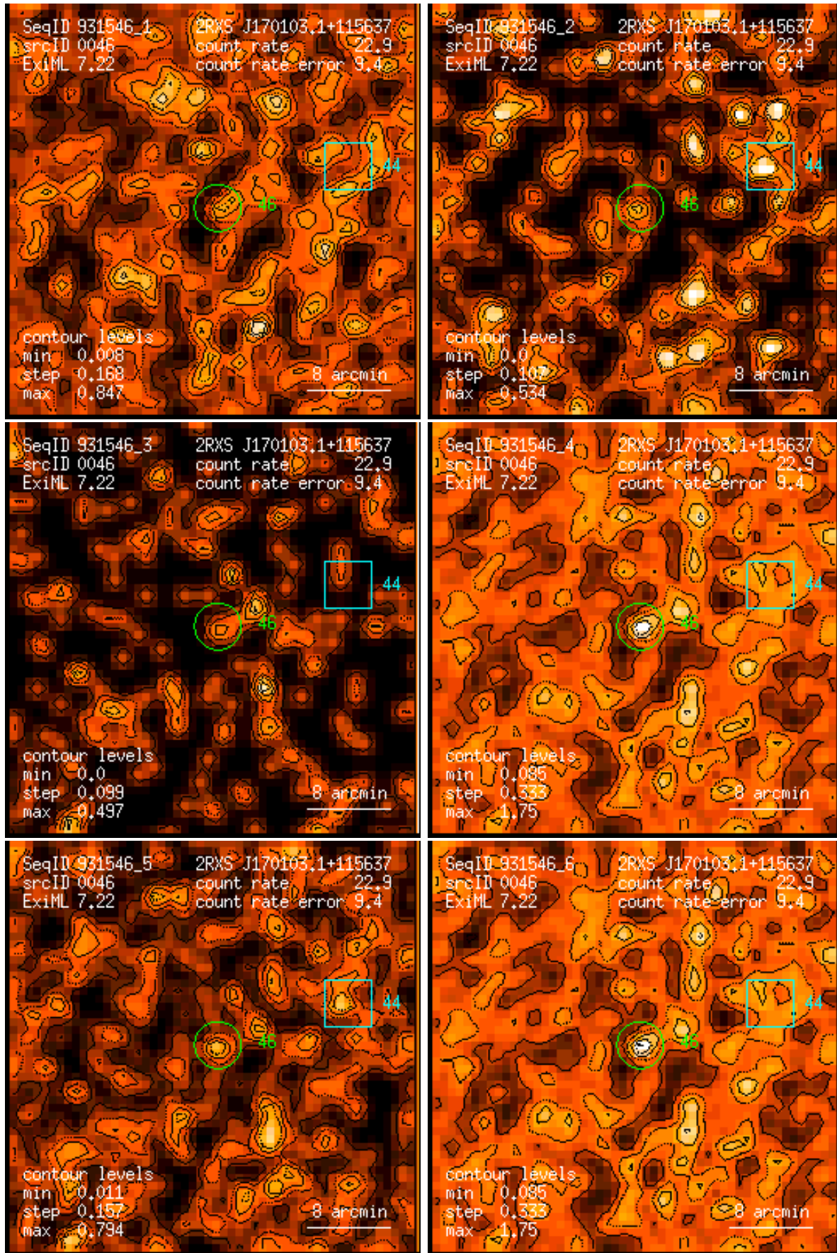
Figure 46: RASS 931546: detection 0046: band rate images, Gaussian filter: (1) PSPC channels 11 – 41, (2) 52 – 90, (3) 91 – 201, (4) 11 – 235, (5) 52 – 201, (6) 11 – 201. Broad band rates in counts/ks. Band rate contour levels in counts/ks/arcmin 2 .
