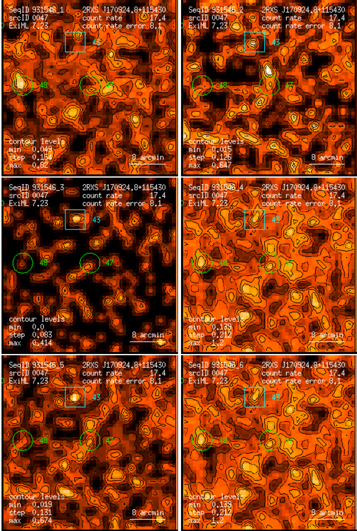
Figure 47: RASS 931546: detection 0047: band rate images, Gaussian filter: (1) PSPC channels 11 – 41, (2) 52 – 90, (3) 91 – 201, (4) 11 – 235, (5) 52 – 201, (6) 11 – 201. Broad band rates in counts/ks. Band rate contour levels in counts/ks/arcmin 2 .
