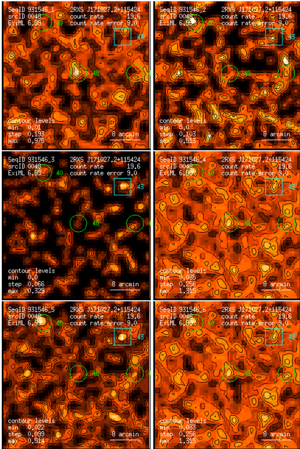
Figure 48: RASS 931546: detection 0048: band rate images, Gaussian filter: (1) PSPC channels 11 – 41, (2) 52 – 90, (3) 91 – 201, (4) 11 – 235, (5) 52 – 201, (6) 11 – 201. Broad band rates in counts/ks. Band rate contour levels in counts/ks/arcmin 2 .
