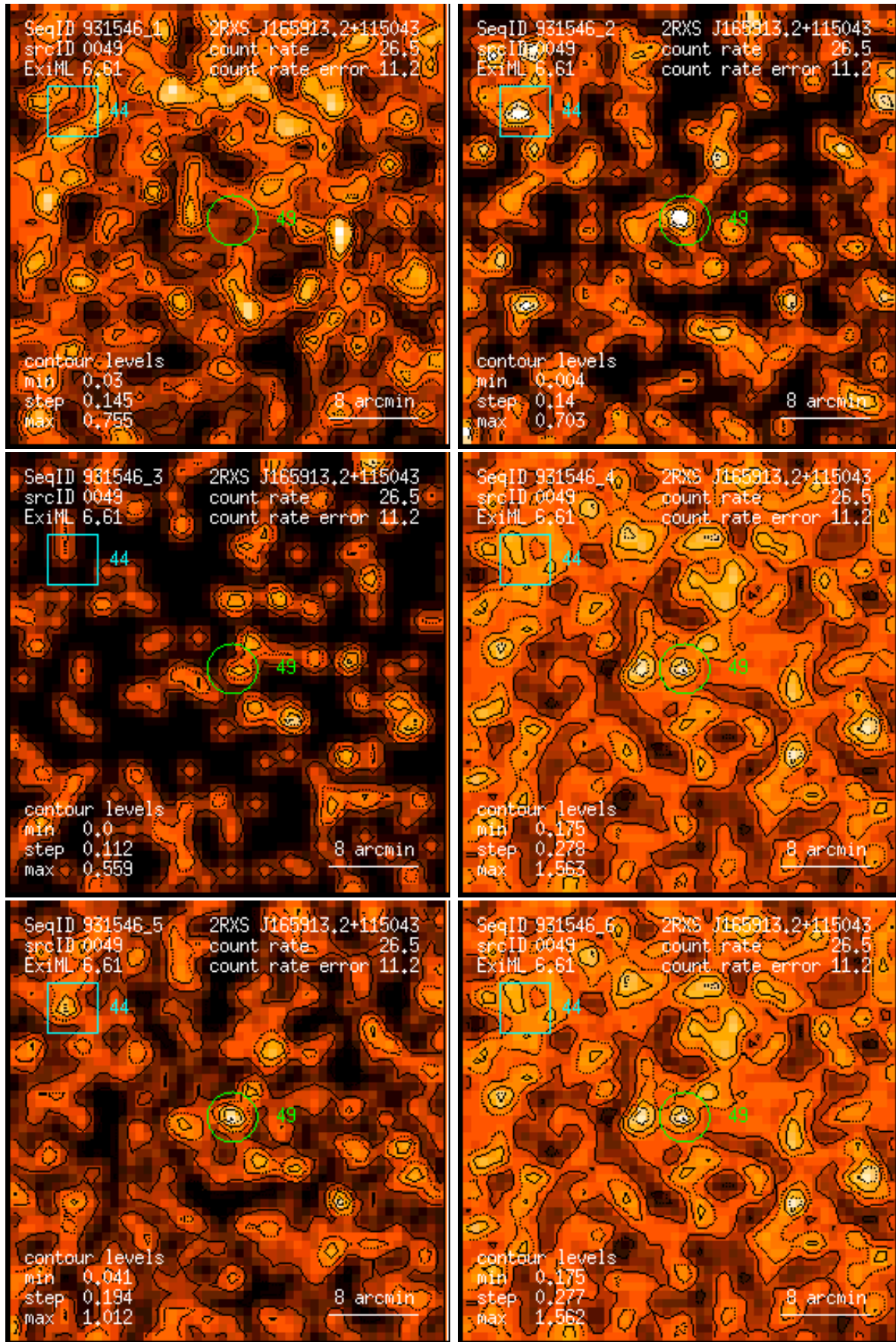
Figure 49: RASS 931546: detection 0049: band rate images, Gaussian filter: (1) PSPC channels 11 – 41, (2) 52 – 90, (3) 91 – 201, (4) 11 – 235, (5) 52 – 201, (6) 11 – 201. Broad band rates in counts/ks. Band rate contour levels in counts/ks/arcmin 2 .
