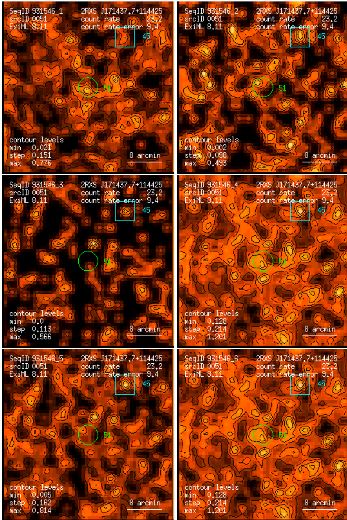
Figure 51: RASS 931546: detection 0051: band rate images, Gaussian filter: (1) PSPC channels 11 – 41, (2) 52 – 90, (3) 91 – 201, (4) 11 – 235, (5) 52 – 201, (6) 11 – 201. Broad band rates in counts/ks. Band rate contour levels in counts/ks/arcmin 2 .
