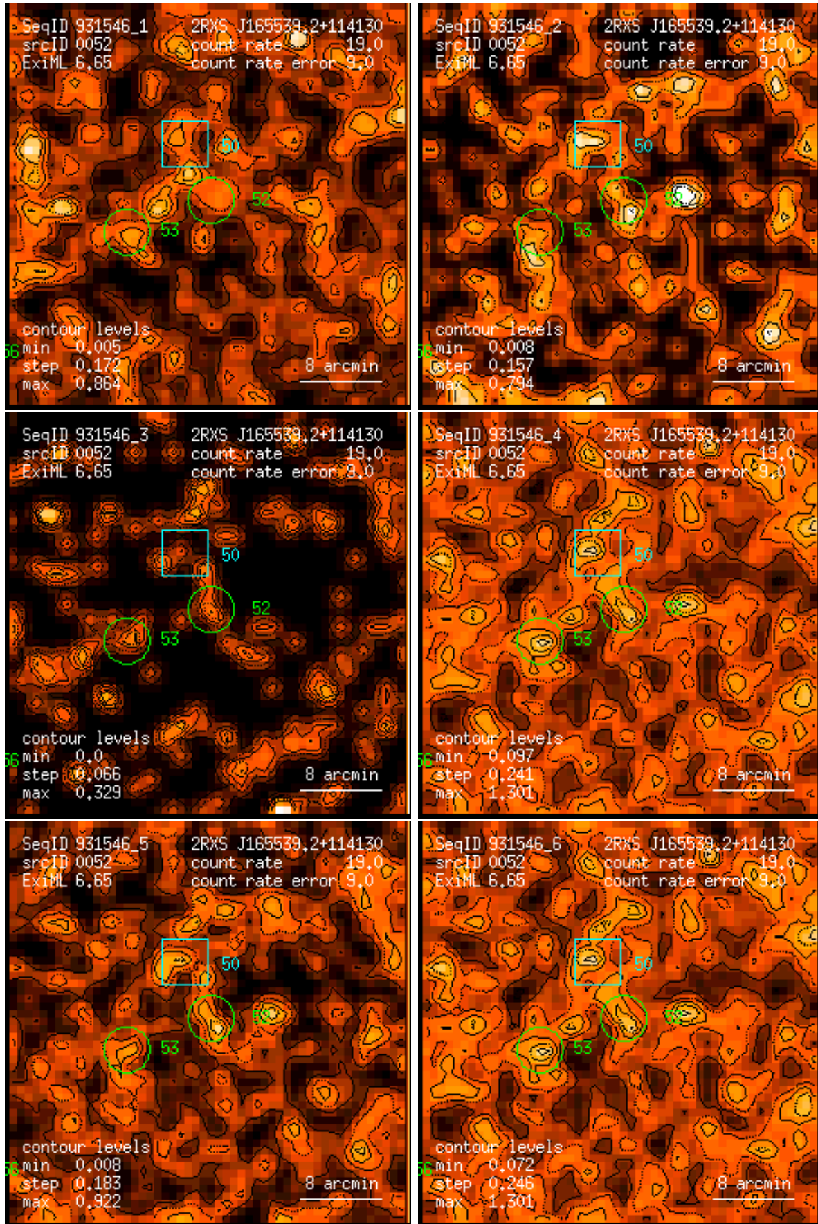
Figure 52: RASS 931546: detection 0052: band rate images, Gaussian filter: (1) PSPC channels 11 – 41, (2) 52 – 90, (3) 91 – 201, (4) 11 – 235, (5) 52 – 201, (6) 11 – 201. Broad band rates in counts/ks. Band rate contour levels in counts/ks/arcmin 2 .
