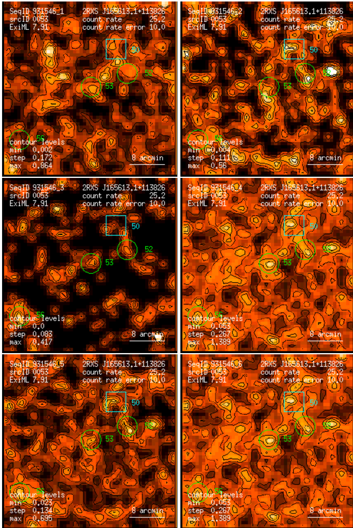
Figure 53: RASS 931546: detection 0053: band rate images, Gaussian filter: (1) PSPC channels 11 – 41, (2) 52 – 90, (3) 91 – 201, (4) 11 – 235, (5) 52 – 201, (6) 11 – 201. Broad band rates in counts/ks. Band rate contour levels in counts/ks/arcmin 2 .
