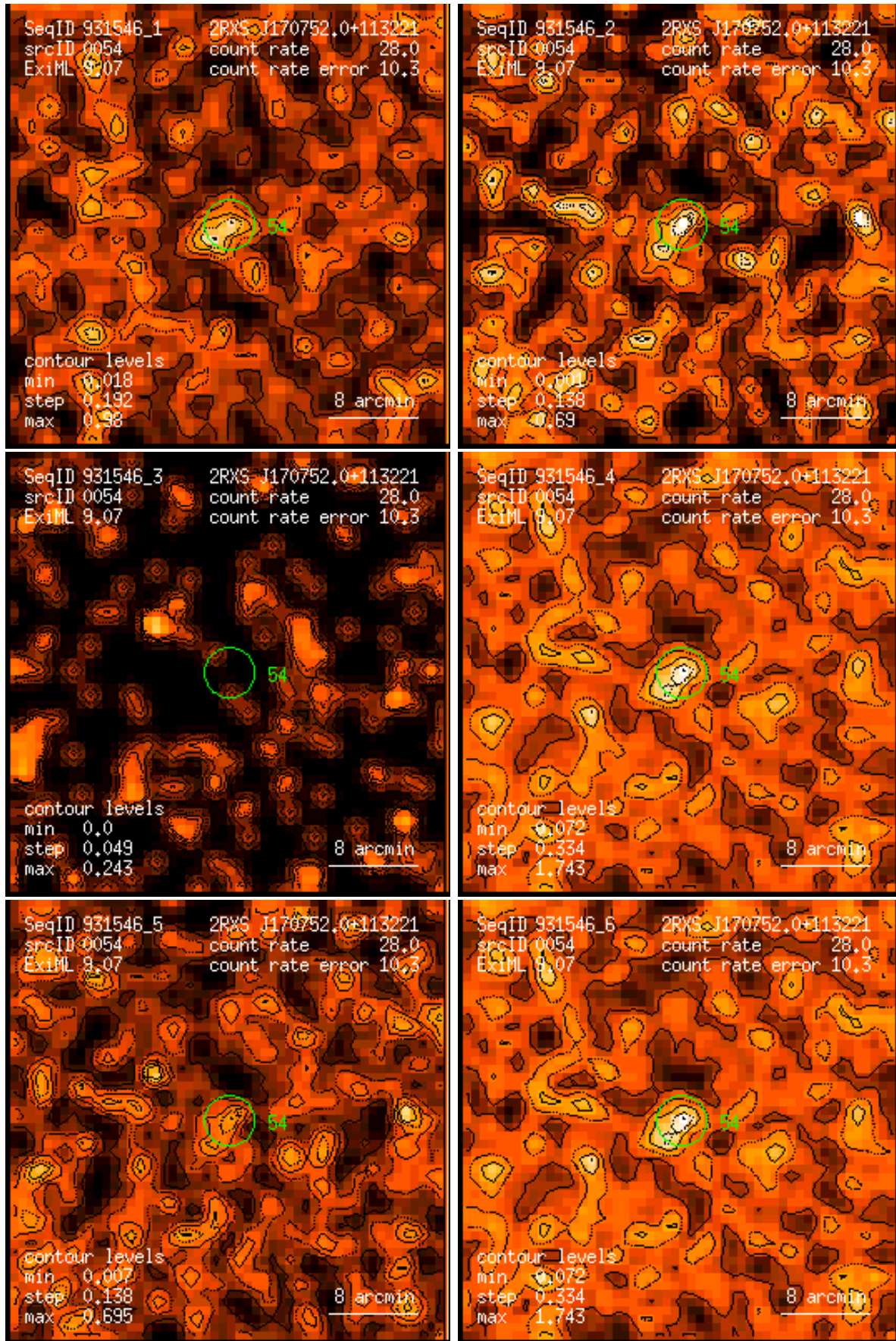
Figure 54: RASS 931546: detection 0054: band rate images, Gaussian filter: (1) PSPC channels 11 – 41, (2) 52 – 90, (3) 91 – 201, (4) 11 – 235, (5) 52 – 201, (6) 11 – 201. Broad band rates in counts/ks. Band rate contour levels in counts/ks/arcmin 2 .
