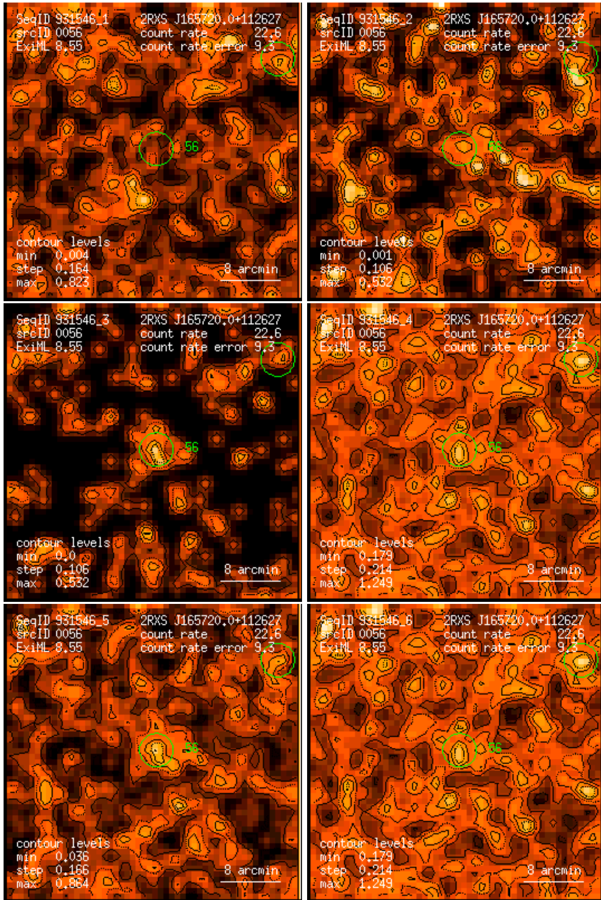
Figure 56: RASS 931546: detection 0056: band rate images, Gaussian filter: (1) PSPC channels 11 – 41, (2) 52 – 90, (3) 91 – 201, (4) 11 – 235, (5) 52 – 201, (6) 11 – 201. Broad band rates in counts/ks. Band rate contour levels in counts/ks/arcmin 2 .
