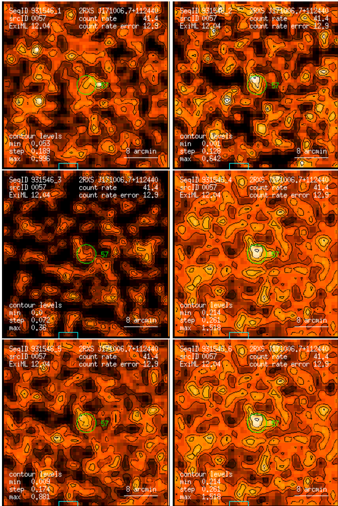
Figure 57: RASS 931546: detection 0057: band rate images, Gaussian filter: (1) PSPC channels 11 – 41, (2) 52 – 90, (3) 91 – 201, (4) 11 – 235, (5) 52 – 201, (6) 11 – 201. Broad band rates in counts/ks. Band rate contour levels in counts/ks/arcmin 2 .
