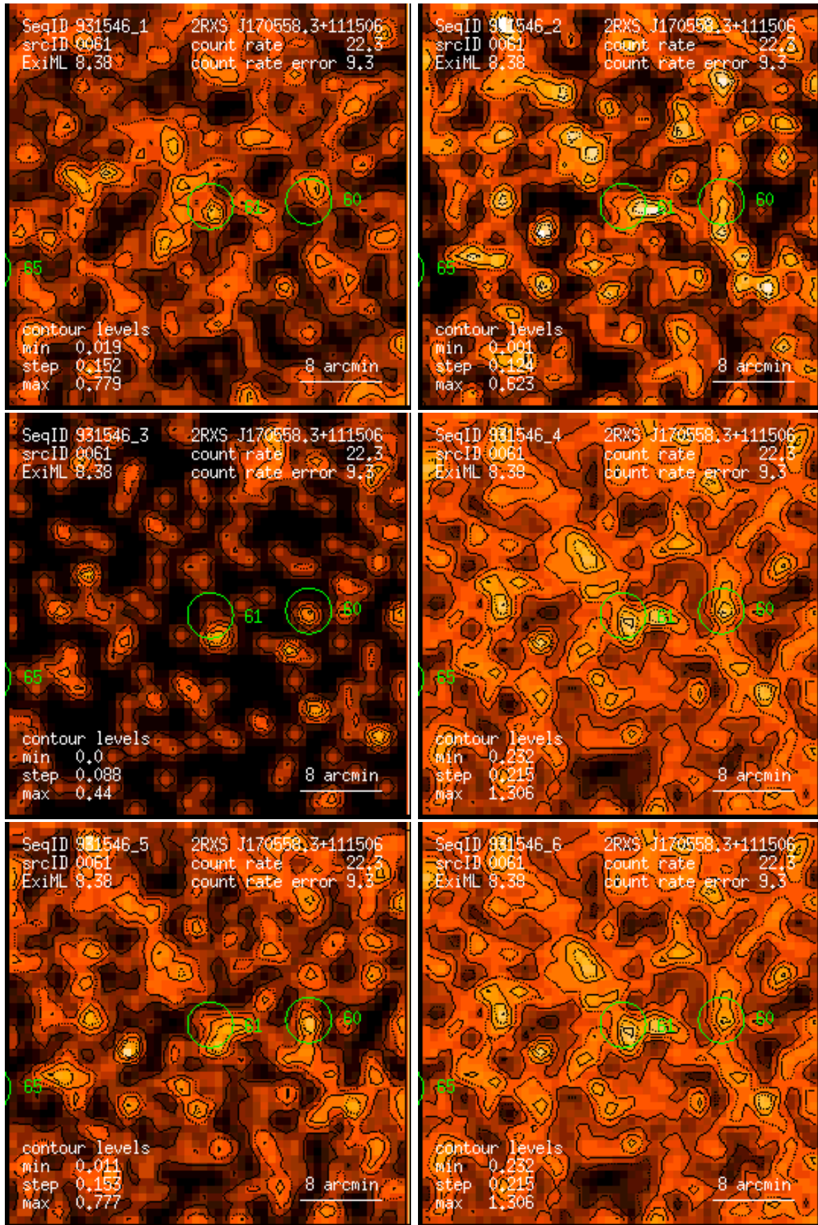
Figure 61: RASS 931546: detection 0061: band rate images, Gaussian filter: (1) PSPC channels 11 – 41, (2) 52 – 90, (3) 91 – 201, (4) 11 – 235, (5) 52 – 201, (6) 11 – 201. Broad band rates in counts/ks. Band rate contour levels in counts/ks/arcmin 2 .
