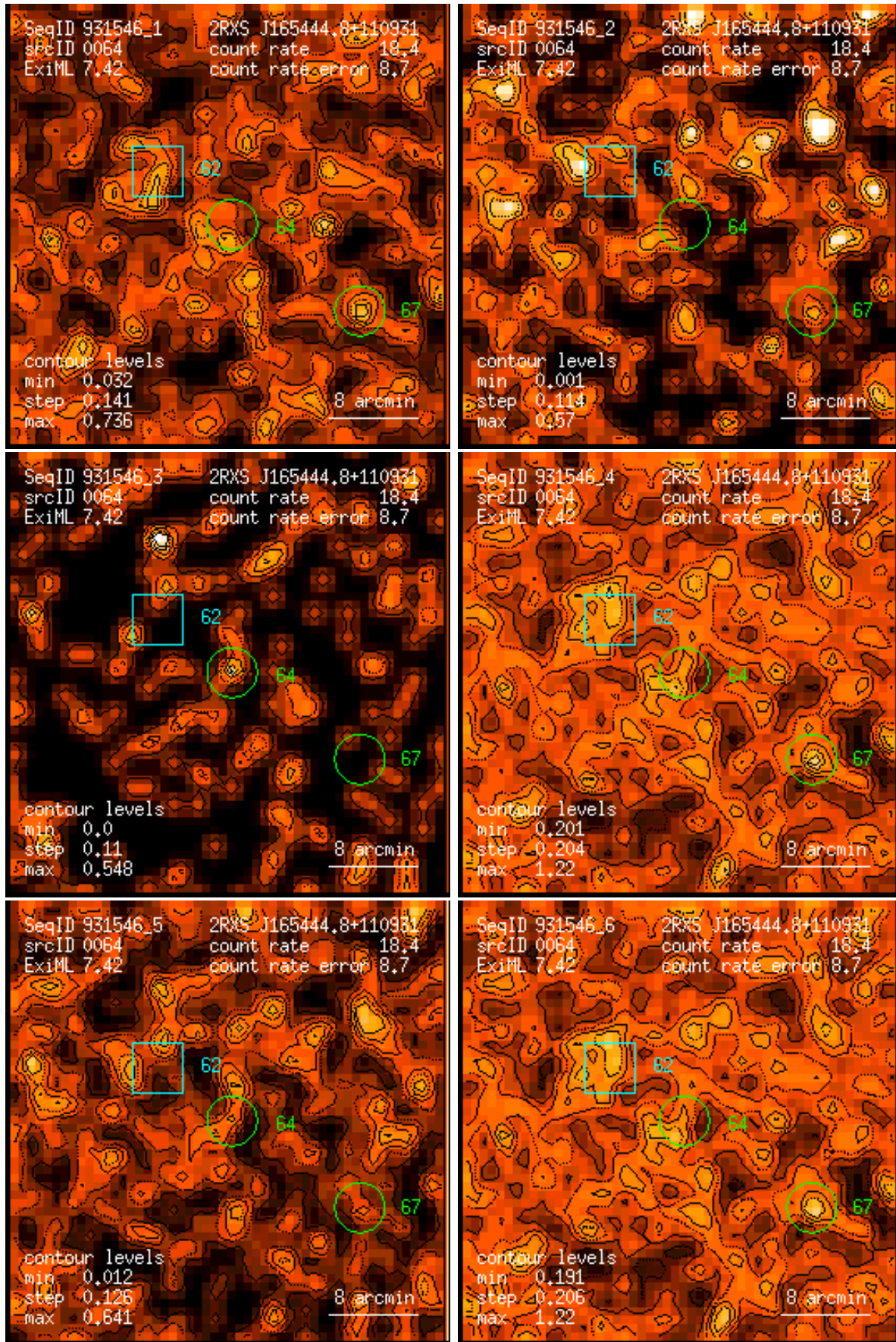
Figure 64: RASS 931546: detection 0064: band rate images, Gaussian filter: (1) PSPC channels 11 – 41, (2) 52 – 90, (3) 91 – 201, (4) 11 – 235, (5) 52 – 201, (6) 11 – 201. Broad band rates in counts/ks. Band rate contour levels in counts/ks/arcmin 2 .
