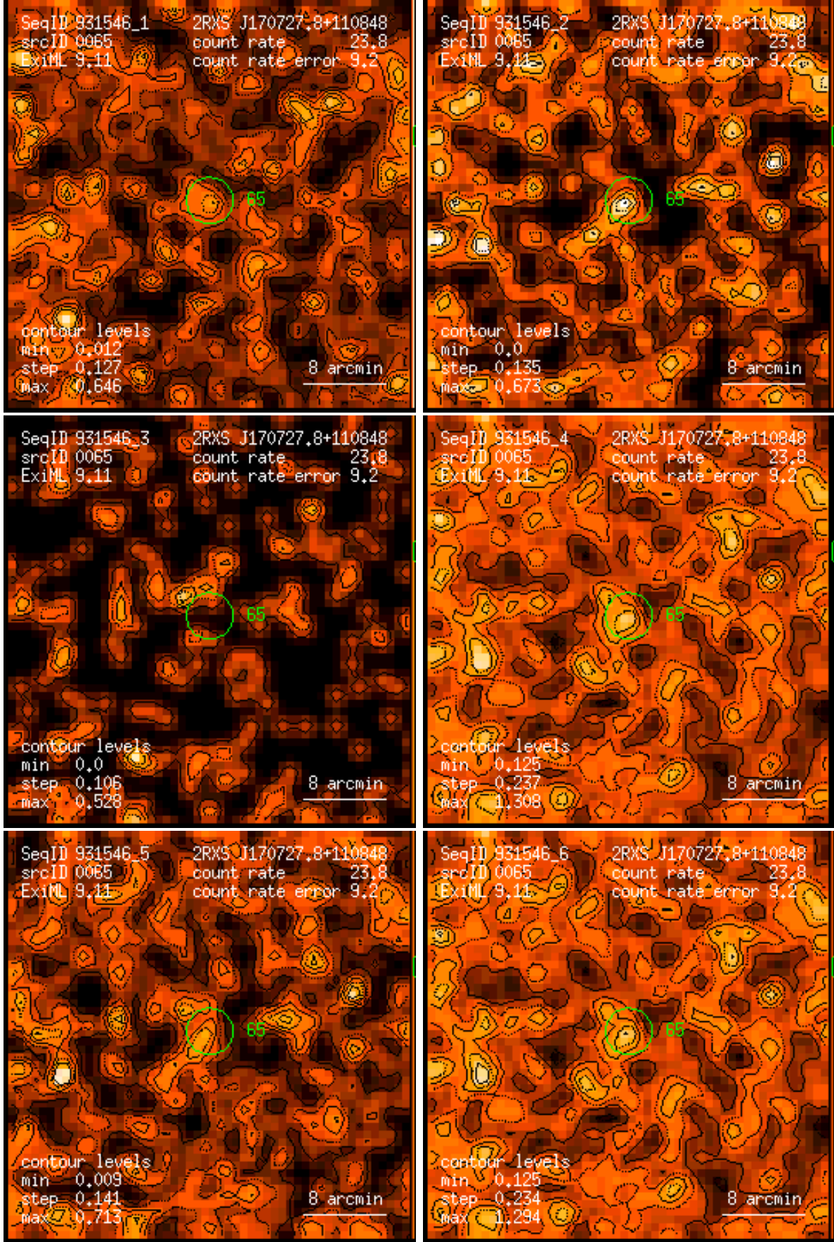
Figure 65: RASS 931546: detection 0065: band rate images, Gaussian filter: (1) PSPC channels 11 – 41, (2) 52 – 90, (3) 91 – 201, (4) 11 – 235, (5) 52 – 201, (6) 11 – 201. Broad band rates in counts/ks. Band rate contour levels in counts/ks/arcmin 2 .
