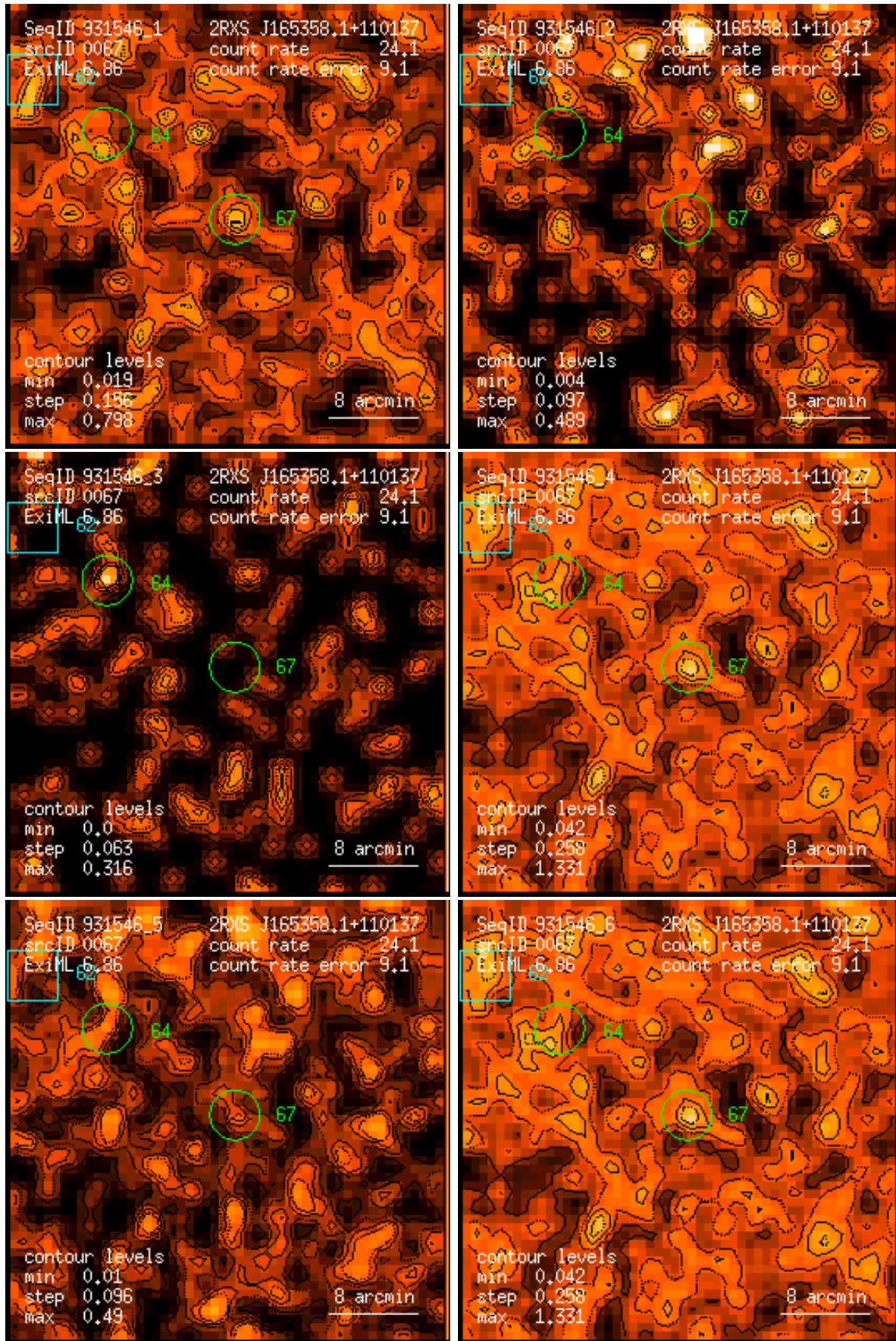
Figure 67: RASS 931546: detection 0067: band rate images, Gaussian filter: (1) PSPC channels 11 – 41, (2) 52 – 90, (3) 91 – 201, (4) 11 – 235, (5) 52 – 201, (6) 11 – 201. Broad band rates in counts/ks. Band rate contour levels in counts/ks/arcmin 2 .
