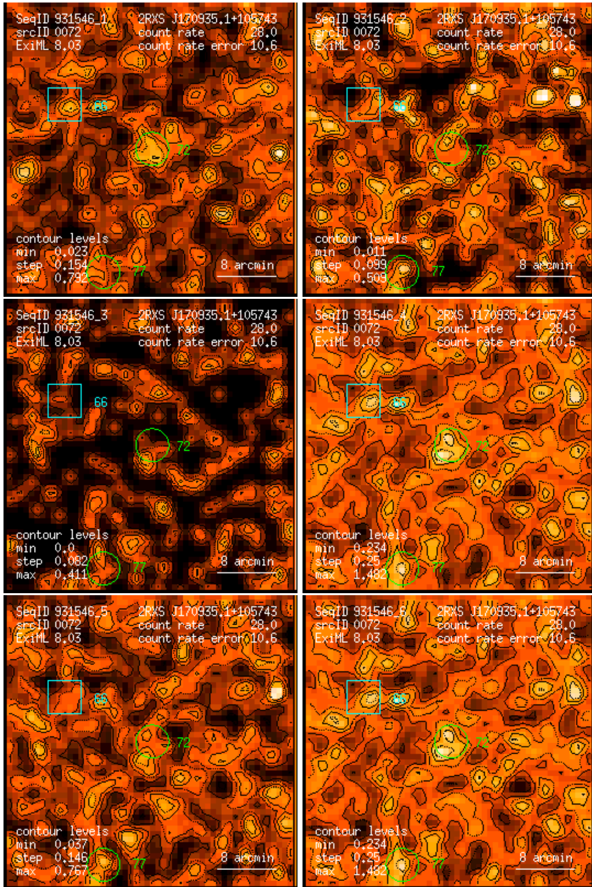
Figure 72: RASS 931546: detection 0072: band rate images, Gaussian filter: (1) PSPC channels 11 – 41, (2) 52 – 90, (3) 91 – 201, (4) 11 – 235, (5) 52 – 201, (6) 11 – 201. Broad band rates in counts/ks. Band rate contour levels in counts/ks/arcmin 2 .
