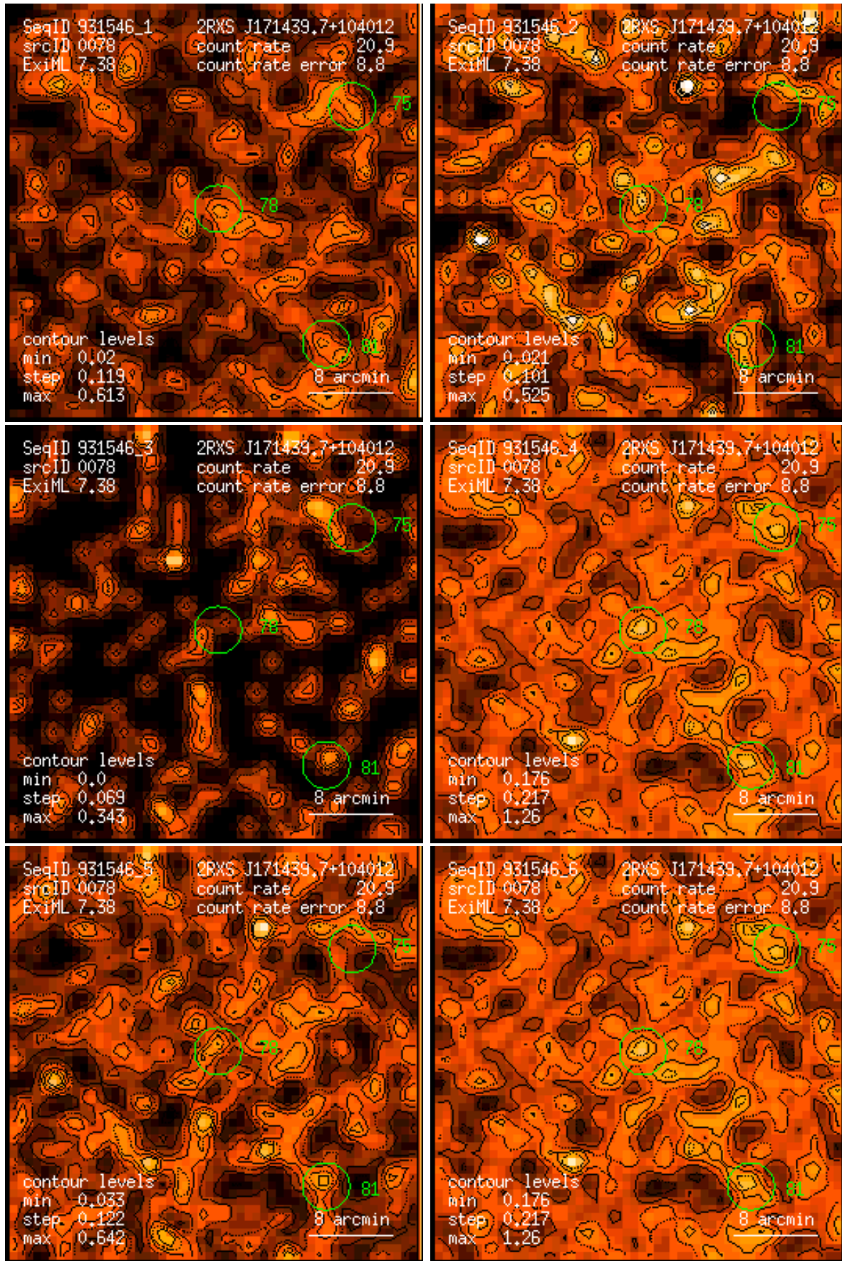
Figure 78: RASS 931546: detection 0078: band rate images, Gaussian filter: (1) PSPC channels 11 – 41, (2) 52 – 90, (3) 91 – 201, (4) 11 – 235, (5) 52 – 201, (6) 11 – 201. Broad band rates in counts/ks. Band rate contour levels in counts/ks/arcmin 2 .
