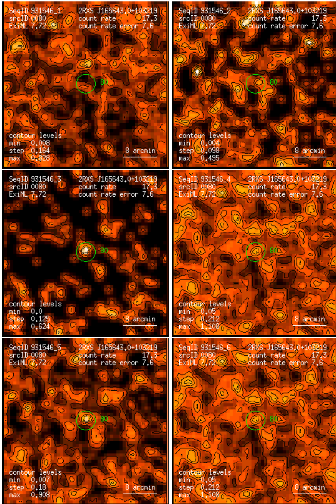
Figure 80: RASS 931546: detection 0080: band rate images, Gaussian filter: (1) PSPC channels 11 – 41, (2) 52 – 90, (3) 91 – 201, (4) 11 – 235, (5) 52 – 201, (6) 11 – 201. Broad band rates in counts/ks. Band rate contour levels in counts/ks/arcmin 2 .
