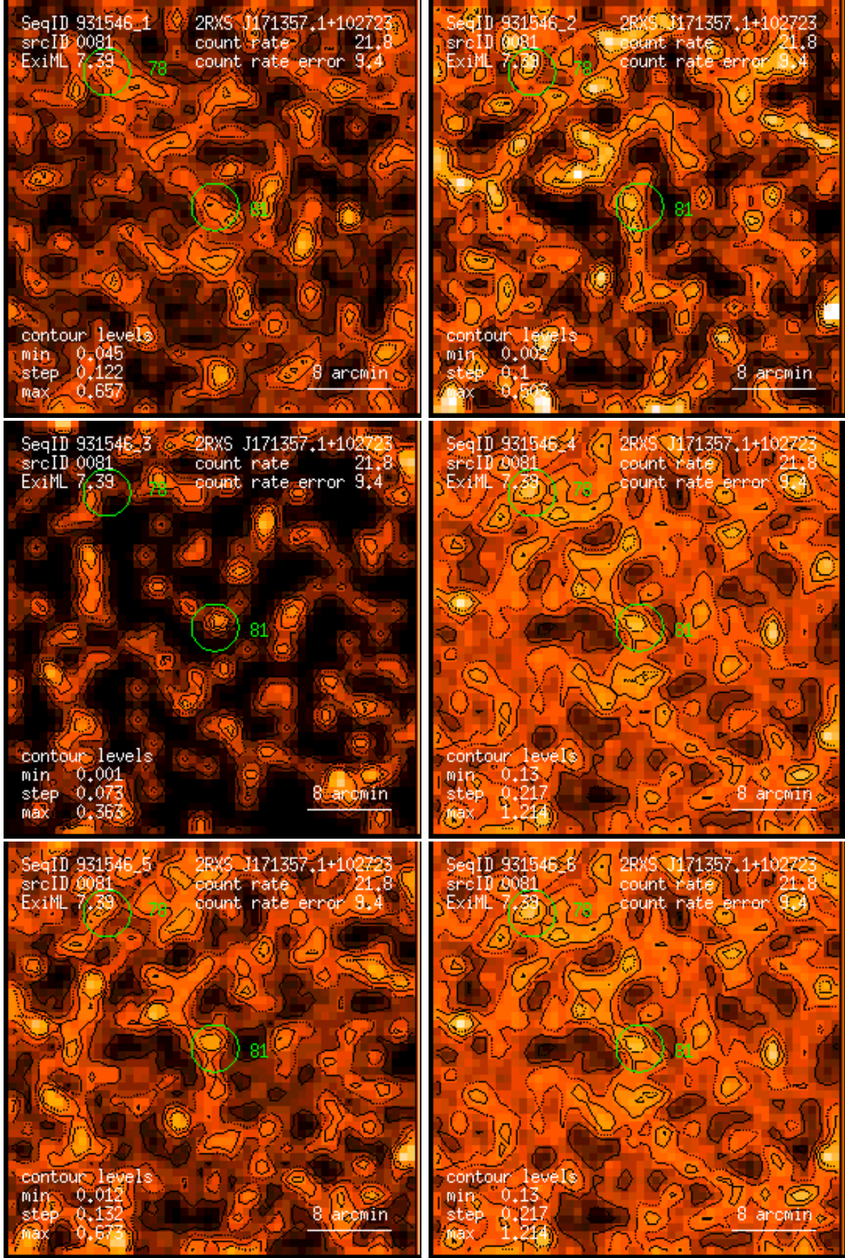
Figure 81: RASS 931546: detection 0081: band rate images, Gaussian filter: (1) PSPC channels 11 – 41, (2) 52 – 90, (3) 91 – 201, (4) 11 – 235, (5) 52 – 201, (6) 11 – 201. Broad band rates in counts/ks. Band rate contour levels in counts/ks/arcmin 2 .
