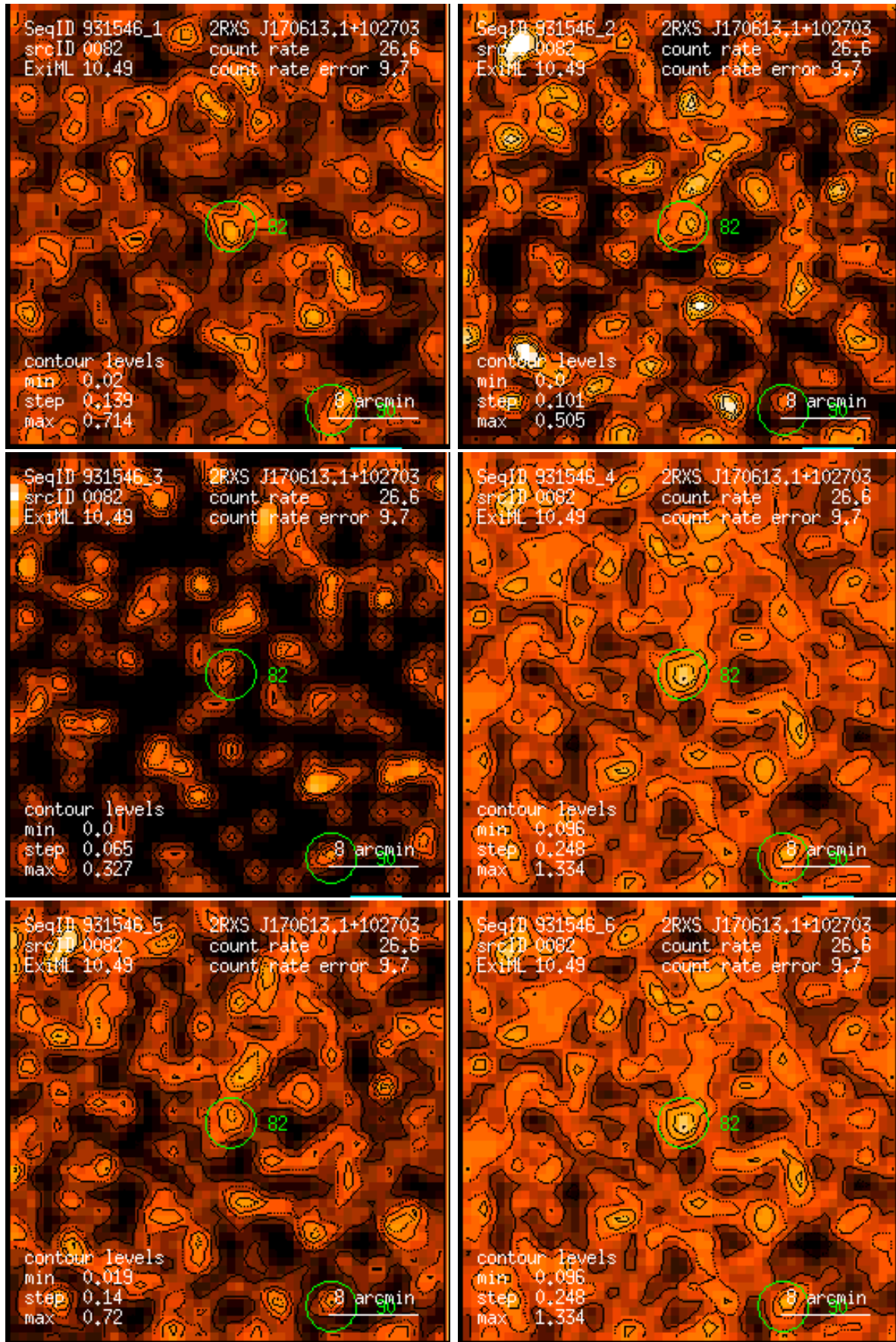
Figure 82: RASS 931546: detection 0082: band rate images, Gaussian filter: (1) PSPC channels 11 – 41, (2) 52 – 90, (3) 91 – 201, (4) 11 – 235, (5) 52 – 201, (6) 11 – 201. Broad band rates in counts/ks. Band rate contour levels in counts/ks/arcmin 2 .
