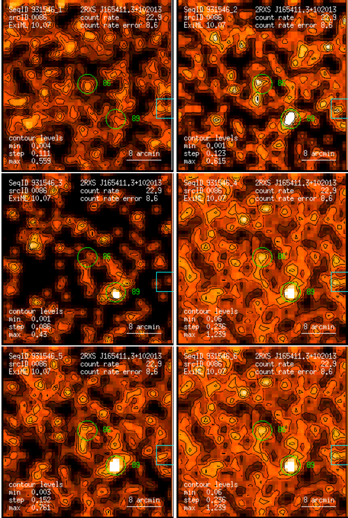
Figure 86: RASS 931546: detection 0086: band rate images, Gaussian filter: (1) PSPC channels 11 – 41, (2) 52 – 90, (3) 91 – 201, (4) 11 – 235, (5) 52 – 201, (6) 11 – 201. Broad band rates in counts/ks. Band rate contour levels in counts/ks/arcmin 2 .
