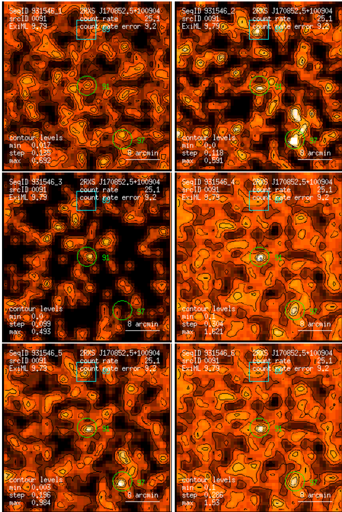
Figure 91: RASS 931546: detection 0091: band rate images, Gaussian filter: (1) PSPC channels 11 – 41, (2) 52 – 90, (3) 91 – 201, (4) 11 – 235, (5) 52 – 201, (6) 11 – 201. Broad band rates in counts/ks. Band rate contour levels in counts/ks/arcmin 2 .
