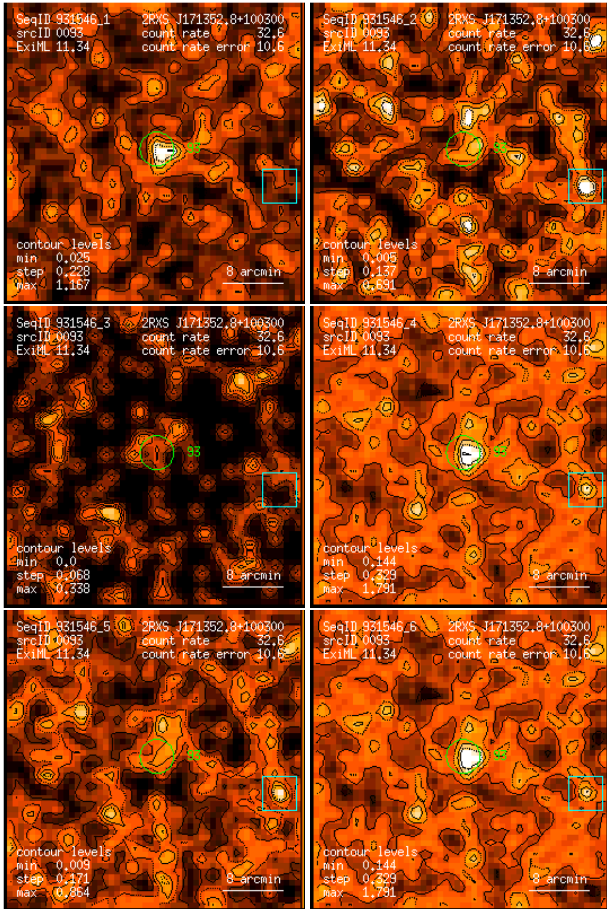
Figure 93: RASS 931546: detection 0093: band rate images, Gaussian filter: (1) PSPC channels 11 – 41, (2) 52 – 90, (3) 91 – 201, (4) 11 – 235, (5) 52 – 201, (6) 11 – 201. Broad band rates in counts/ks. Band rate contour levels in counts/ks/arcmin 2 .
