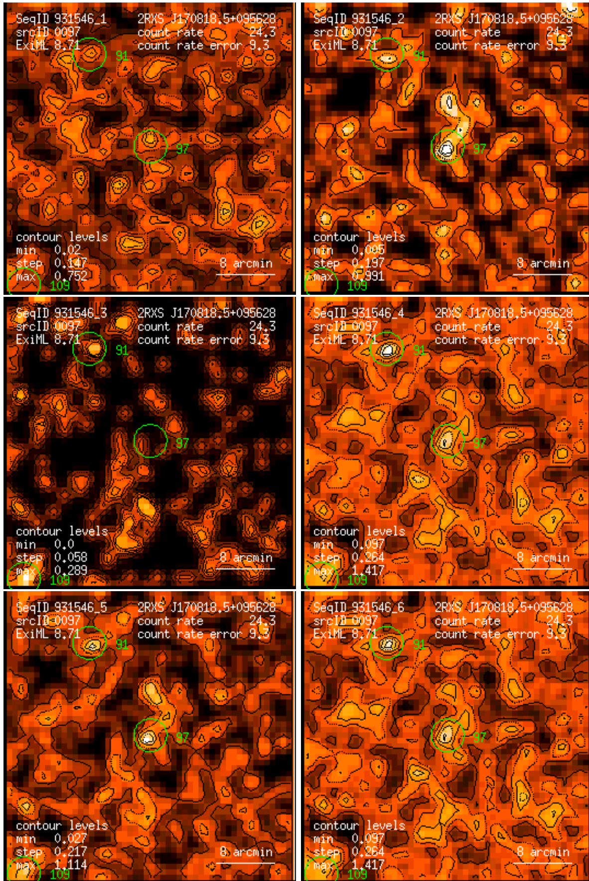
Figure 97: RASS 931546: detection 0097: band rate images, Gaussian filter: (1) PSPC channels 11 – 41, (2) 52 – 90, (3) 91 – 201, (4) 11 – 235, (5) 52 – 201, (6) 11 – 201. Broad band rates in counts/ks. Band rate contour levels in counts/ks/arcmin 2 .
