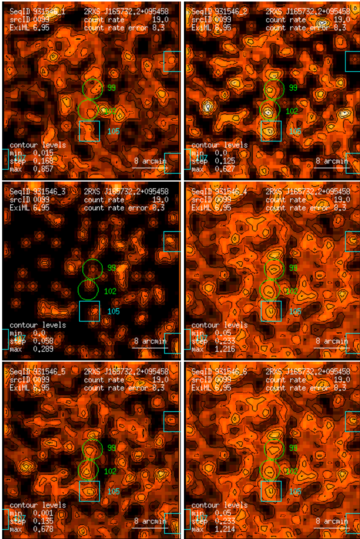
Figure 99: RASS 931546: detection 0099: band rate images, Gaussian filter: (1) PSPC channels 11 – 41, (2) 52 – 90, (3) 91 – 201, (4) 11 – 235, (5) 52 – 201, (6) 11 – 201. Broad band rates in counts/ks. Band rate contour levels in counts/ks/arcmin 2 .
