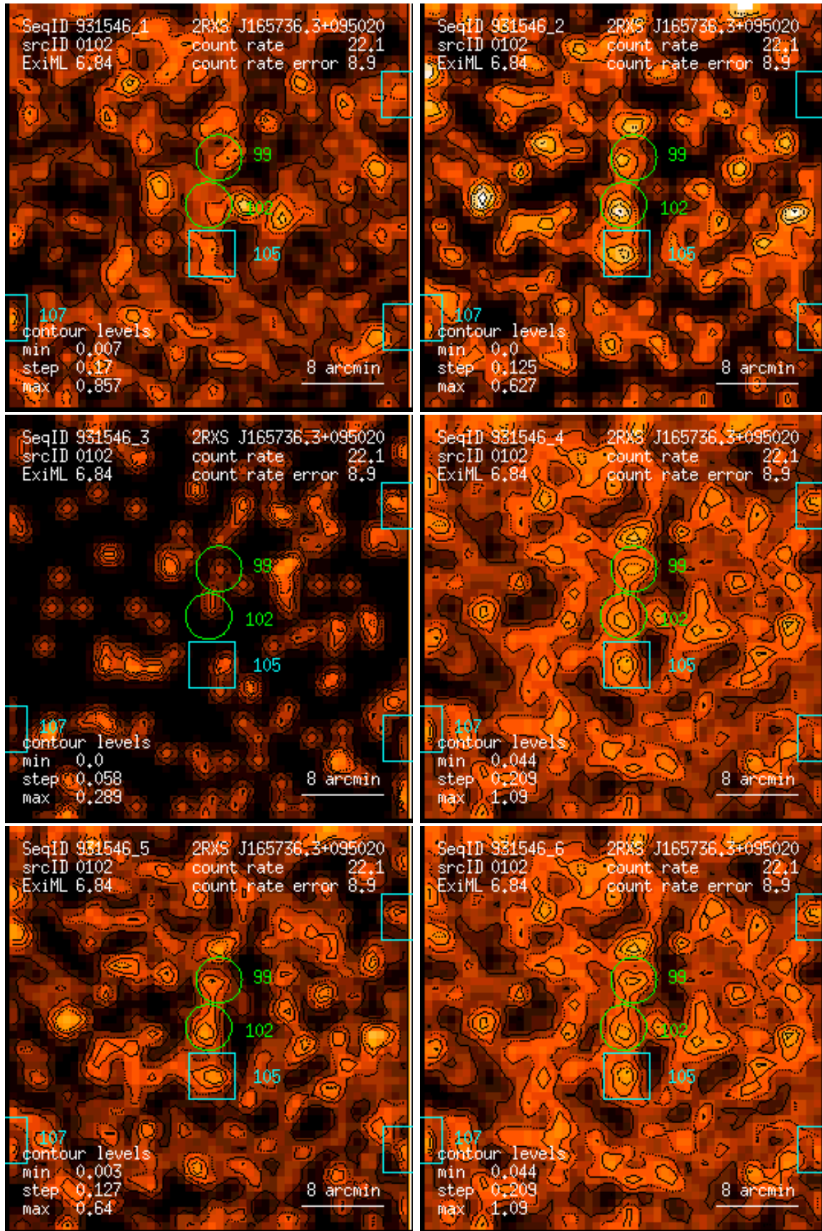
Figure 102: RASS 931546: detection 0102: band rate images, Gaussian filter: (1) PSPC channels 11 – 41, (2) 52 – 90, (3) 91 – 201, (4) 11 – 235, (5) 52 – 201, (6) 11 – 201. Broad band rates in counts/ks. Band rate contour levels in counts/ks/arcmin 2 .
