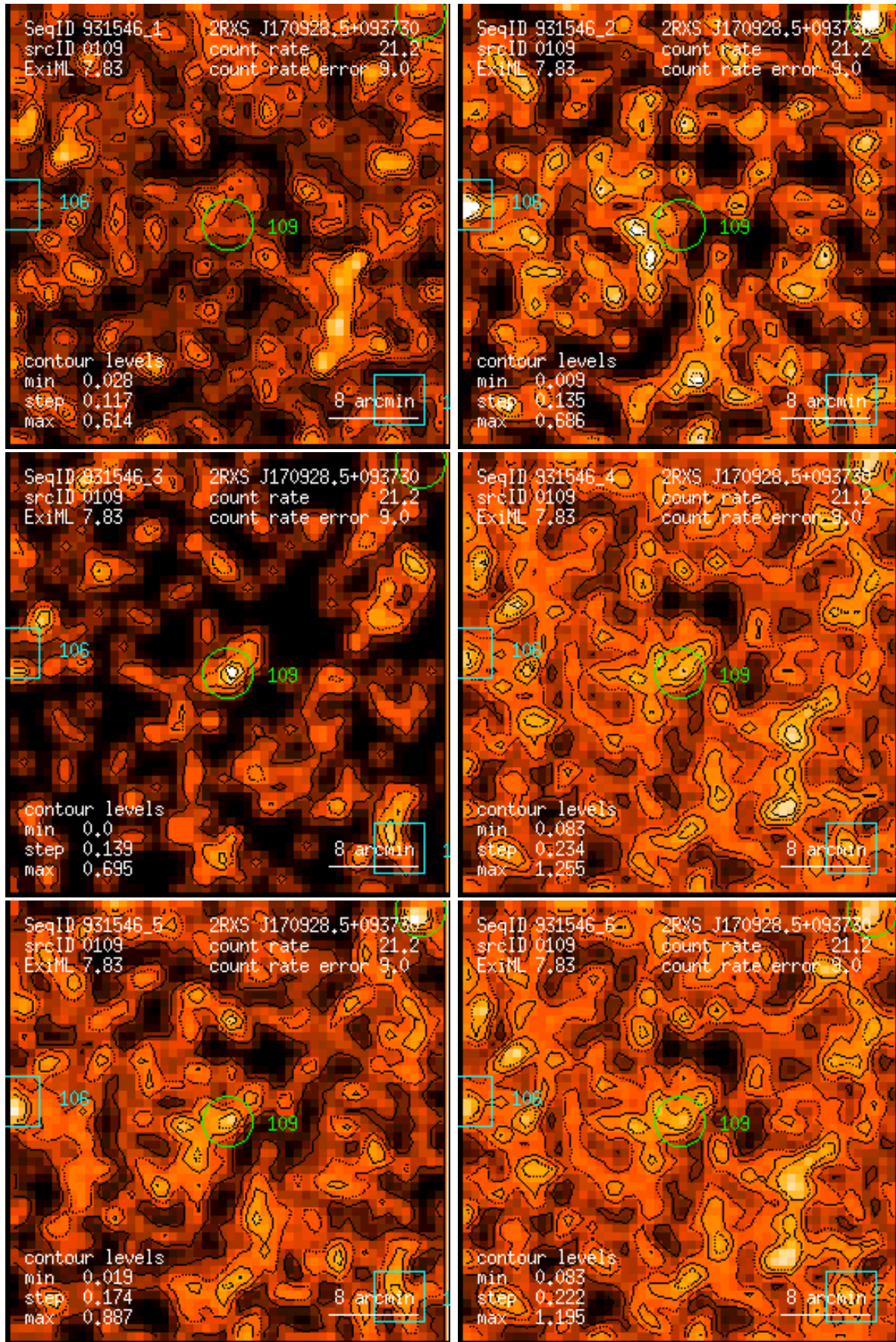
Figure 109: RASS 931546: detection 0109: band rate images, Gaussian filter: (1) PSPC channels 11 – 41, (2) 52 – 90, (3) 91 – 201, (4) 11 – 235, (5) 52 – 201, (6) 11 – 201. Broad band rates in counts/ks. Band rate contour levels in counts/ks/arcmin 2 .
