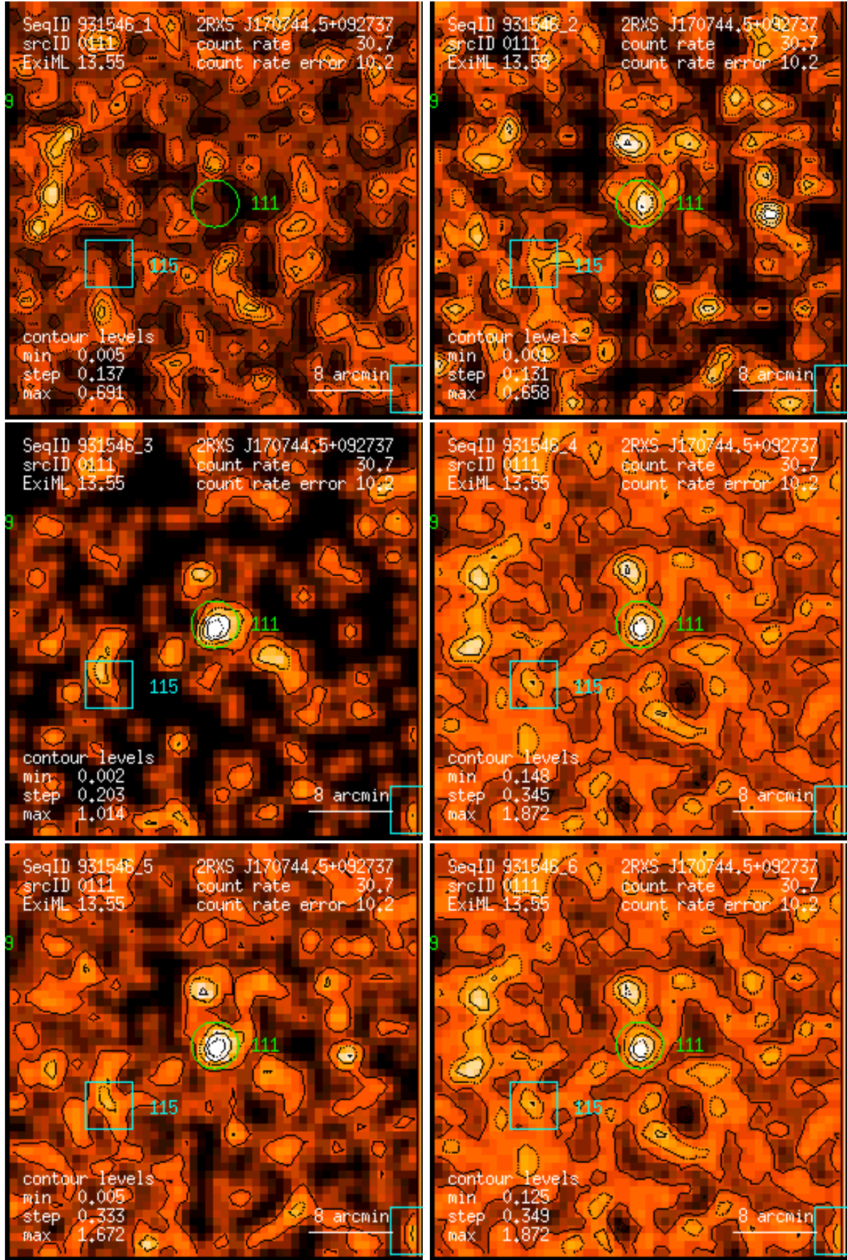
Figure 111: RASS 931546: detection 0111: band rate images, Gaussian filter: (1) PSPC channels 11 – 41, (2) 52 – 90, (3) 91 – 201, (4) 11 – 235, (5) 52 – 201, (6) 11 – 201. Broad band rates in counts/ks. Band rate contour levels in counts/ks/arcmin 2 .
