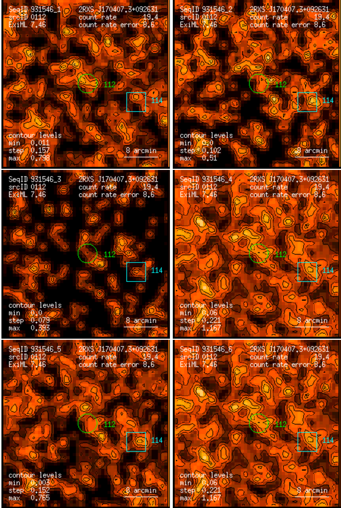
Figure 112: RASS 931546: detection 0112: band rate images, Gaussian filter: (1) PSPC channels 11 – 41, (2) 52 – 90, (3) 91 – 201, (4) 11 – 235, (5) 52 – 201, (6) 11 – 201. Broad band rates in counts/ks. Band rate contour levels in counts/ks/arcmin 2 .
