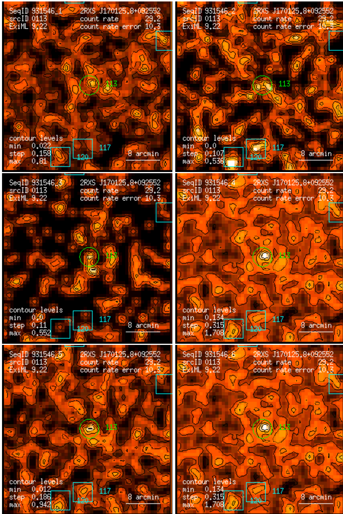
Figure 113: RASS 931546: detection 0113: band rate images, Gaussian filter: (1) PSPC channels 11 – 41, (2) 52 – 90, (3) 91 – 201, (4) 11 – 235, (5) 52 – 201, (6) 11 – 201. Broad band rates in counts/ks. Band rate contour levels in counts/ks/arcmin 2 .
