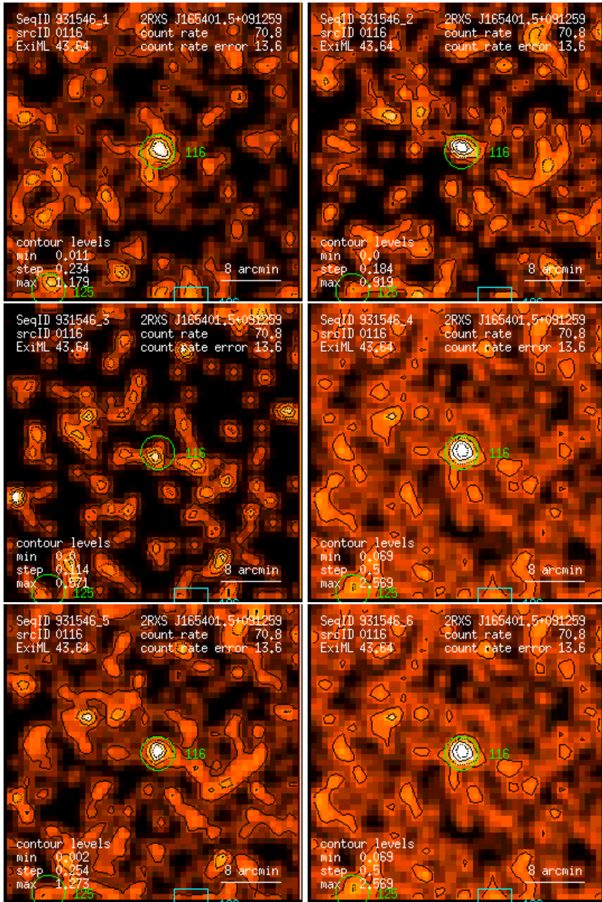
Figure 116: RASS 931546: detection 0116: band rate images, Gaussian filter: (1) PSPC channels 11 – 41, (2) 52 – 90, (3) 91 – 201, (4) 11 – 235, (5) 52 – 201, (6) 11 – 201. Broad band rates in counts/ks. Band rate contour levels in counts/ks/arcmin 2 .
