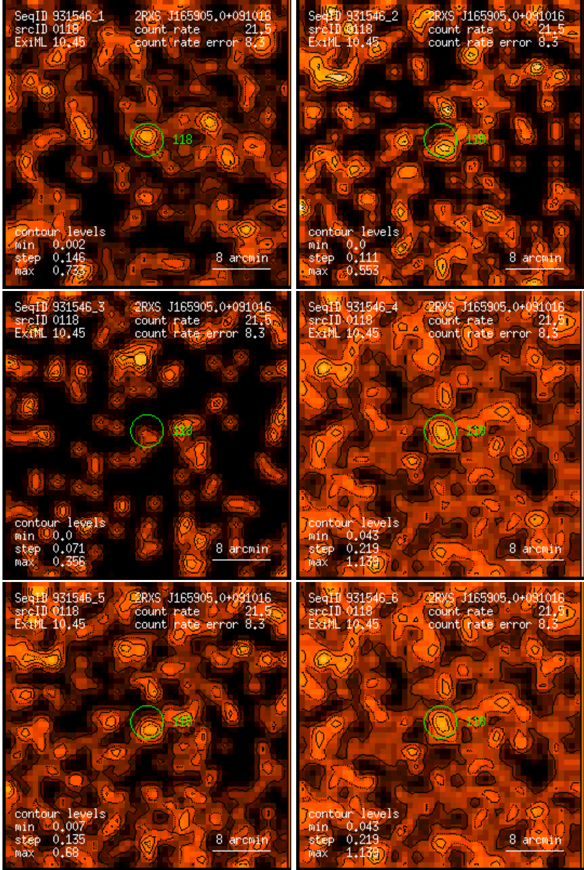
Figure 118: RASS 931546: detection 0118: band rate images, Gaussian filter: (1) PSPC channels 11 – 41, (2) 52 – 90, (3) 91 – 201, (4) 11 – 235, (5) 52 – 201, (6) 11 – 201. Broad band rates in counts/ks. Band rate contour levels in counts/ks/arcmin 2 .
