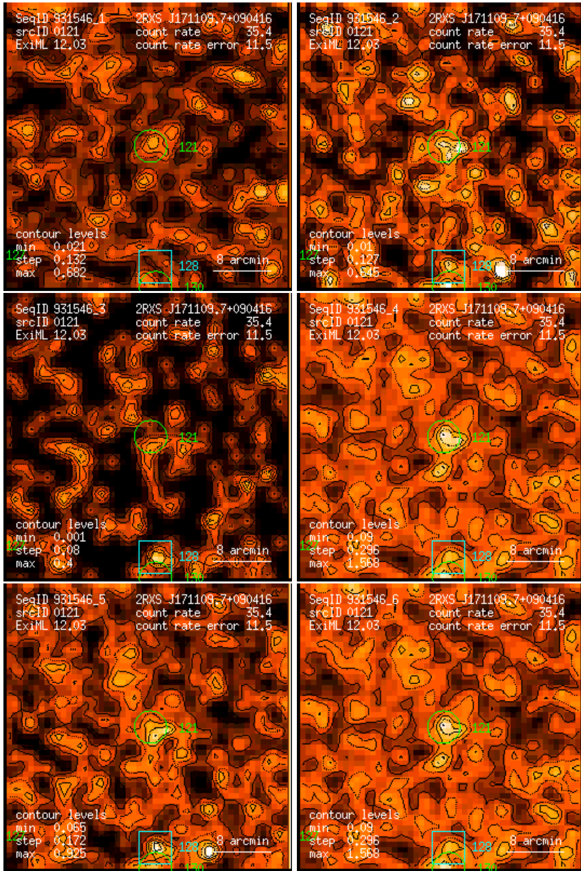
Figure 121: RASS 931546: detection 0121: band rate images, Gaussian filter: (1) PSPC channels 11 – 41, (2) 52 – 90, (3) 91 – 201, (4) 11 – 235, (5) 52 – 201, (6) 11 – 201. Broad band rates in counts/ks. Band rate contour levels in counts/ks/arcmin 2 .
