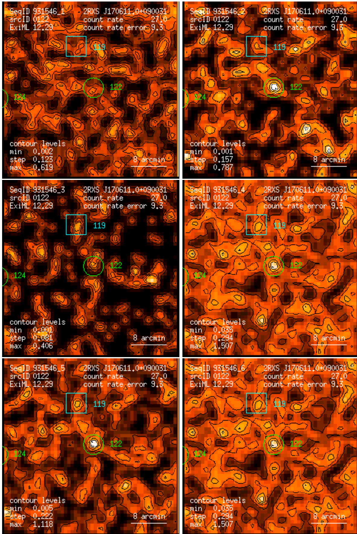
Figure 122: RASS 931546: detection 0122: band rate images, Gaussian filter: (1) PSPC channels 11 – 41, (2) 52 – 90, (3) 91 – 201, (4) 11 – 235, (5) 52 – 201, (6) 11 – 201. Broad band rates in counts/ks. Band rate contour levels in counts/ks/arcmin 2 .
