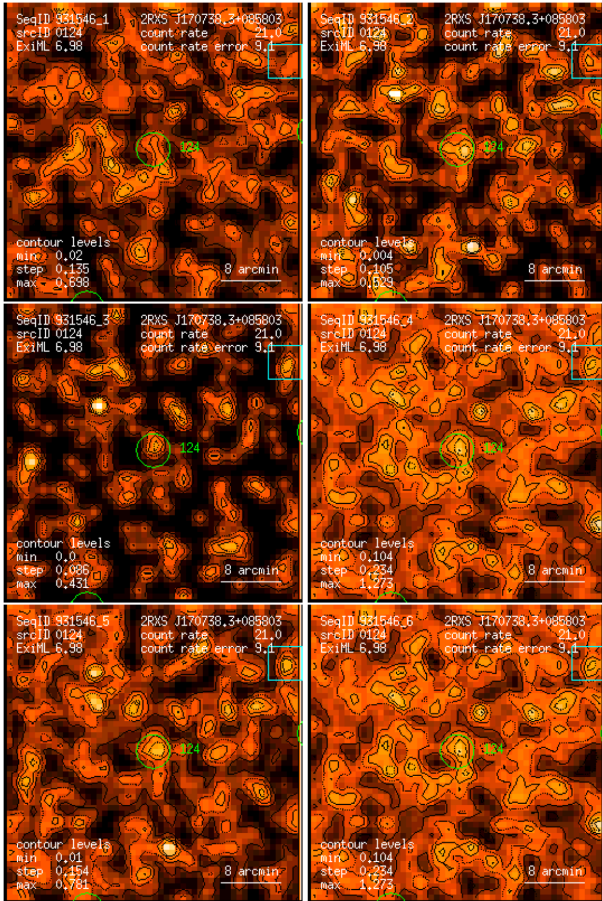
Figure 124: RASS 931546: detection 0124: band rate images, Gaussian filter: (1) PSPC channels 11 – 41, (2) 52 – 90, (3) 91 – 201, (4) 11 – 235, (5) 52 – 201, (6) 11 – 201. Broad band rates in counts/ks. Band rate contour levels in counts/ks/arcmin 2 .
