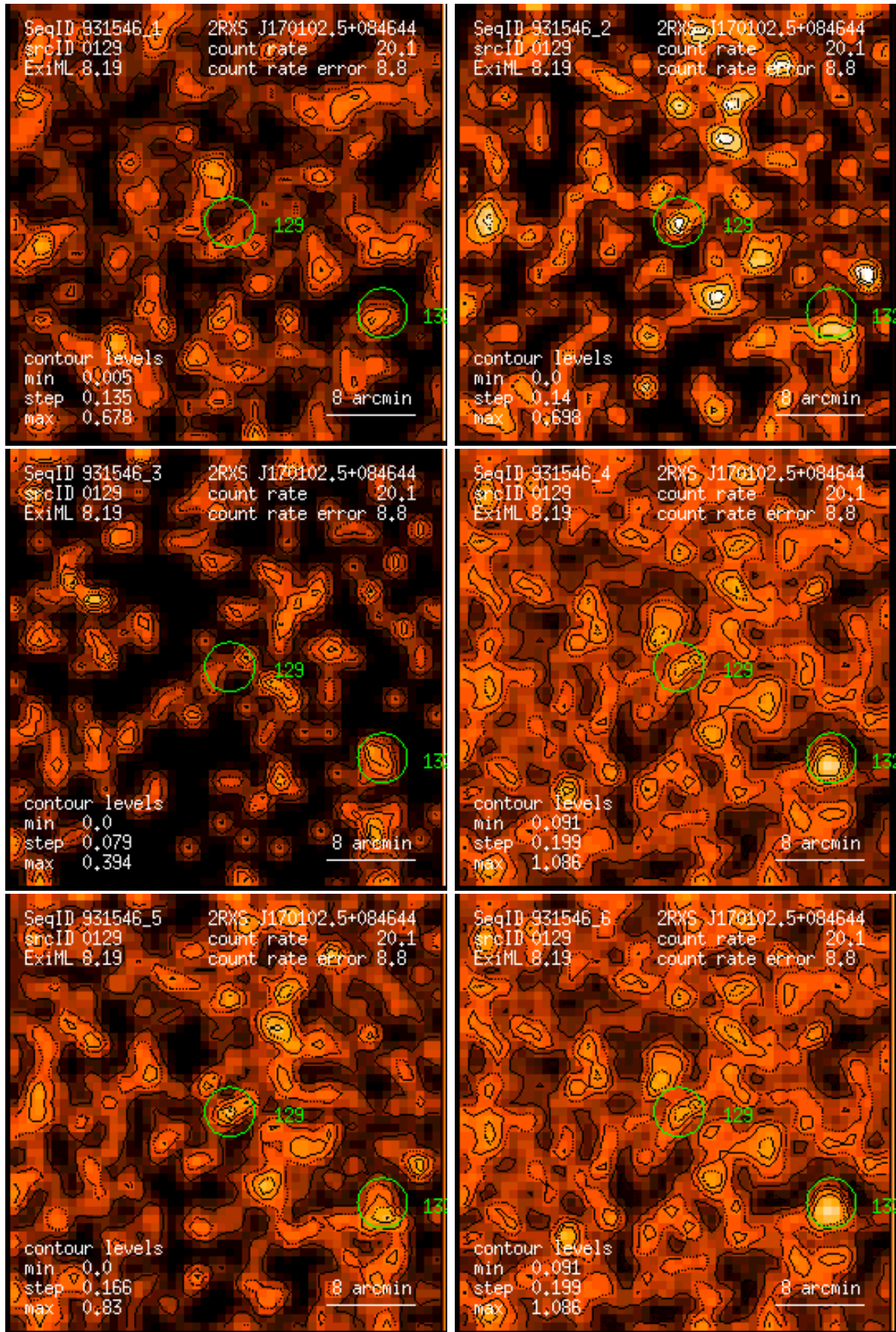
Figure 129: RASS 931546: detection 0129: band rate images, Gaussian filter: (1) PSPC channels 11 – 41, (2) 52 – 90, (3) 91 – 201, (4) 11 – 235, (5) 52 – 201, (6) 11 – 201. Broad band rates in counts/ks. Band rate contour levels in counts/ks/arcmin 2 .
