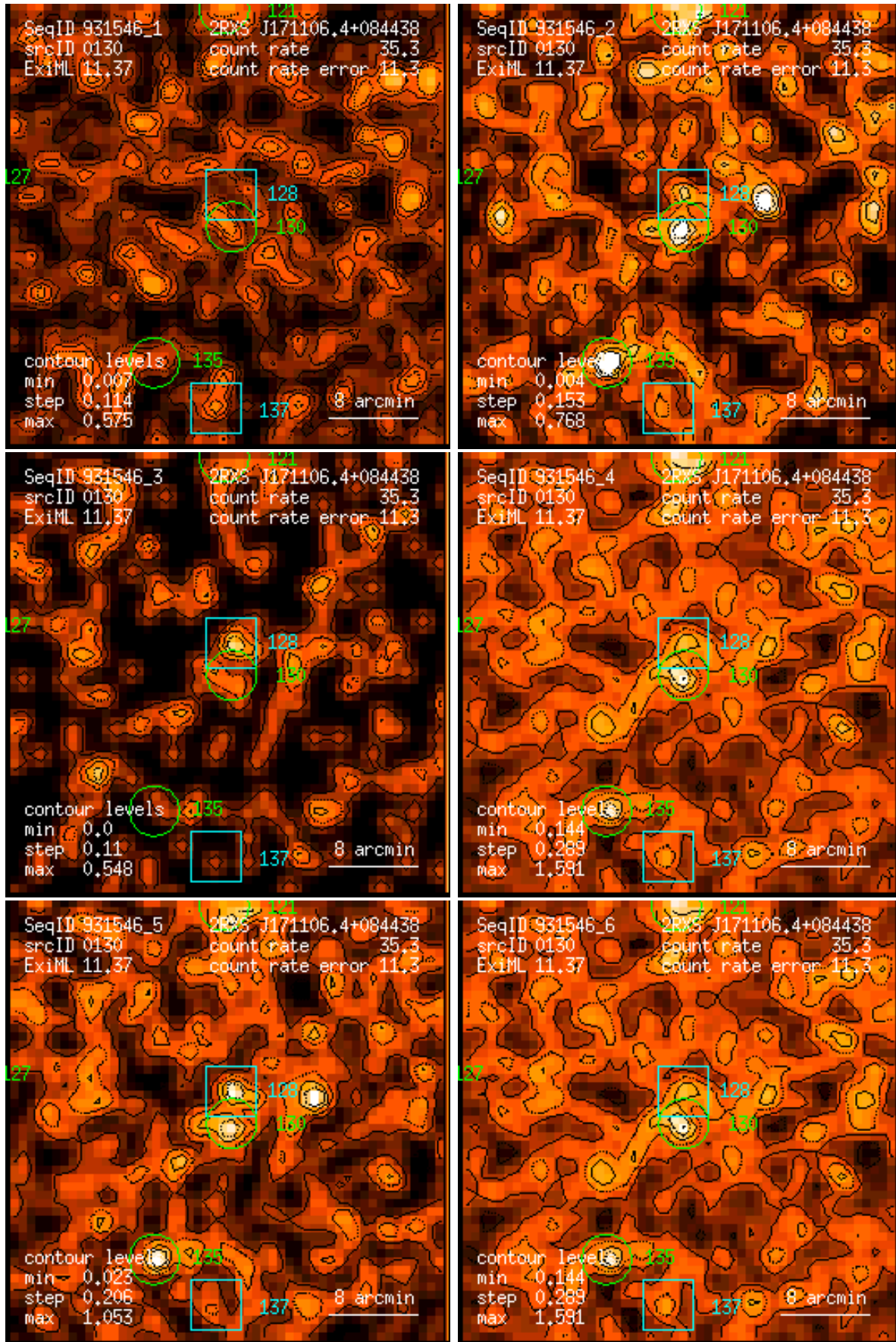
Figure 130: RASS 931546: detection 0130: band rate images, Gaussian filter: (1) PSPC channels 11 – 41, (2) 52 – 90, (3) 91 – 201, (4) 11 – 235, (5) 52 – 201, (6) 11 – 201. Broad band rates in counts/ks. Band rate contour levels in counts/ks/arcmin 2 .
