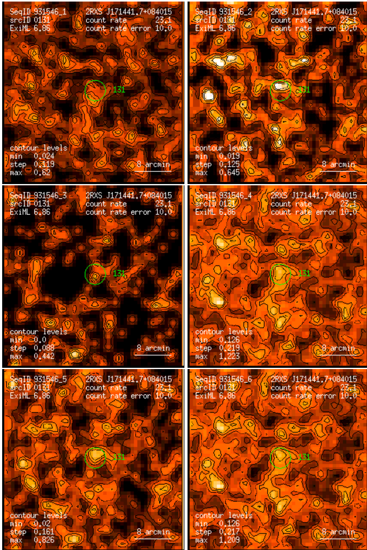
Figure 131: RASS 931546: detection 0131: band rate images, Gaussian filter: (1) PSPC channels 11 – 41, (2) 52 – 90, (3) 91 – 201, (4) 11 – 235, (5) 52 – 201, (6) 11 – 201. Broad band rates in counts/ks. Band rate contour levels in counts/ks/arcmin 2 .
