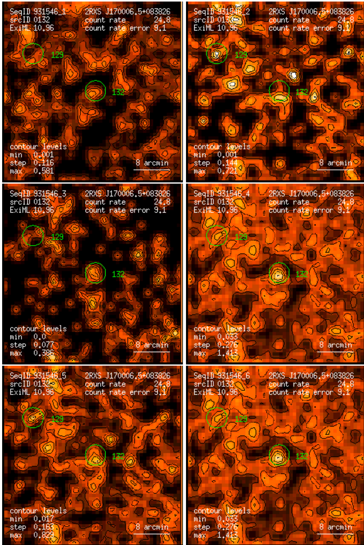
Figure 132: RASS 931546: detection 0132: band rate images, Gaussian filter: (1) PSPC channels 11 – 41, (2) 52 – 90, (3) 91 – 201, (4) 11 – 235, (5) 52 – 201, (6) 11 – 201. Broad band rates in counts/ks. Band rate contour levels in counts/ks/arcmin 2 .
