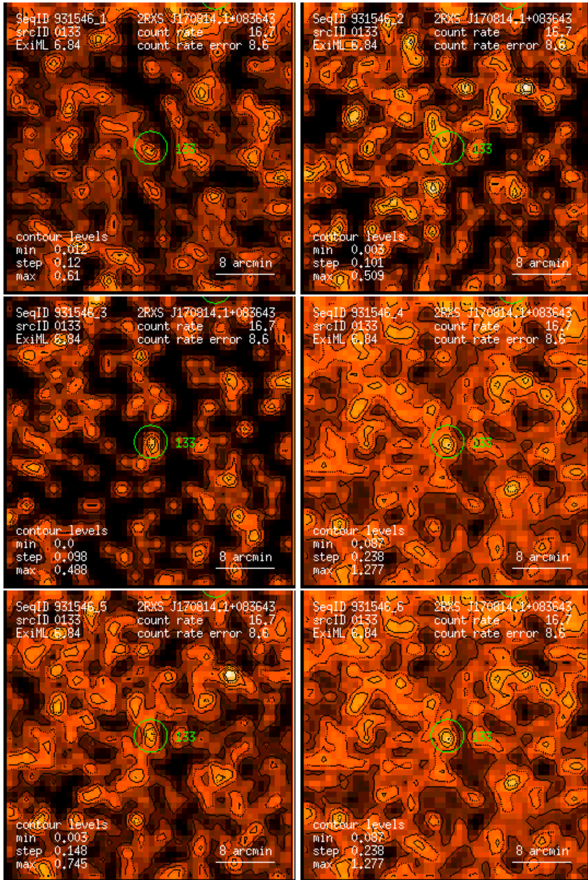
Figure 133: RASS 931546: detection 0133: band rate images, Gaussian filter: (1) PSPC channels 11 – 41, (2) 52 – 90, (3) 91 – 201, (4) 11 – 235, (5) 52 – 201, (6) 11 – 201. Broad band rates in counts/ks. Band rate contour levels in counts/ks/arcmin 2 .
