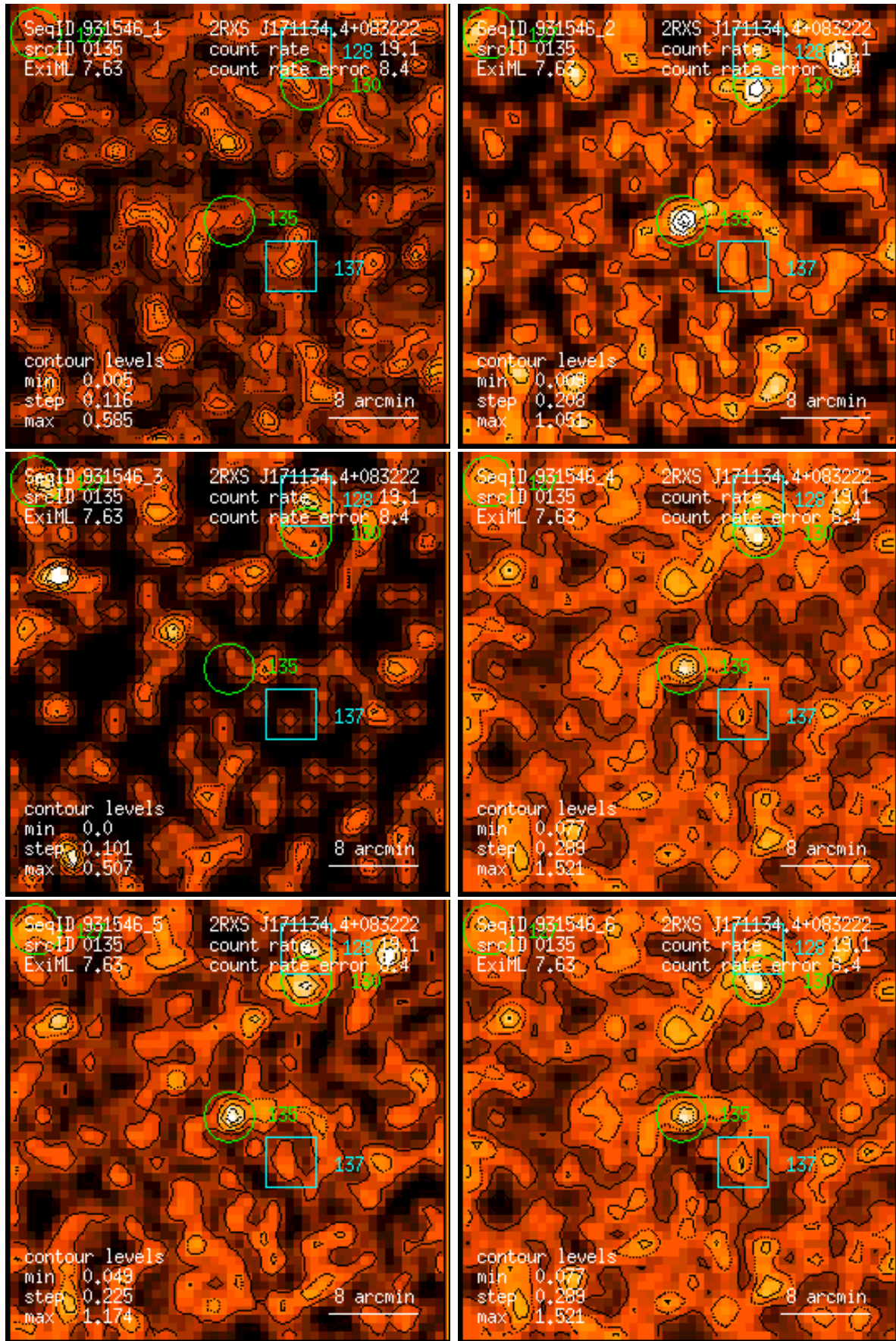
Figure 135: RASS 931546: detection 0135: band rate images, Gaussian filter: (1) PSPC channels 11 – 41, (2) 52 – 90, (3) 91 – 201, (4) 11 – 235, (5) 52 – 201, (6) 11 – 201. Broad band rates in counts/ks. Band rate contour levels in counts/ks/arcmin 2 .
