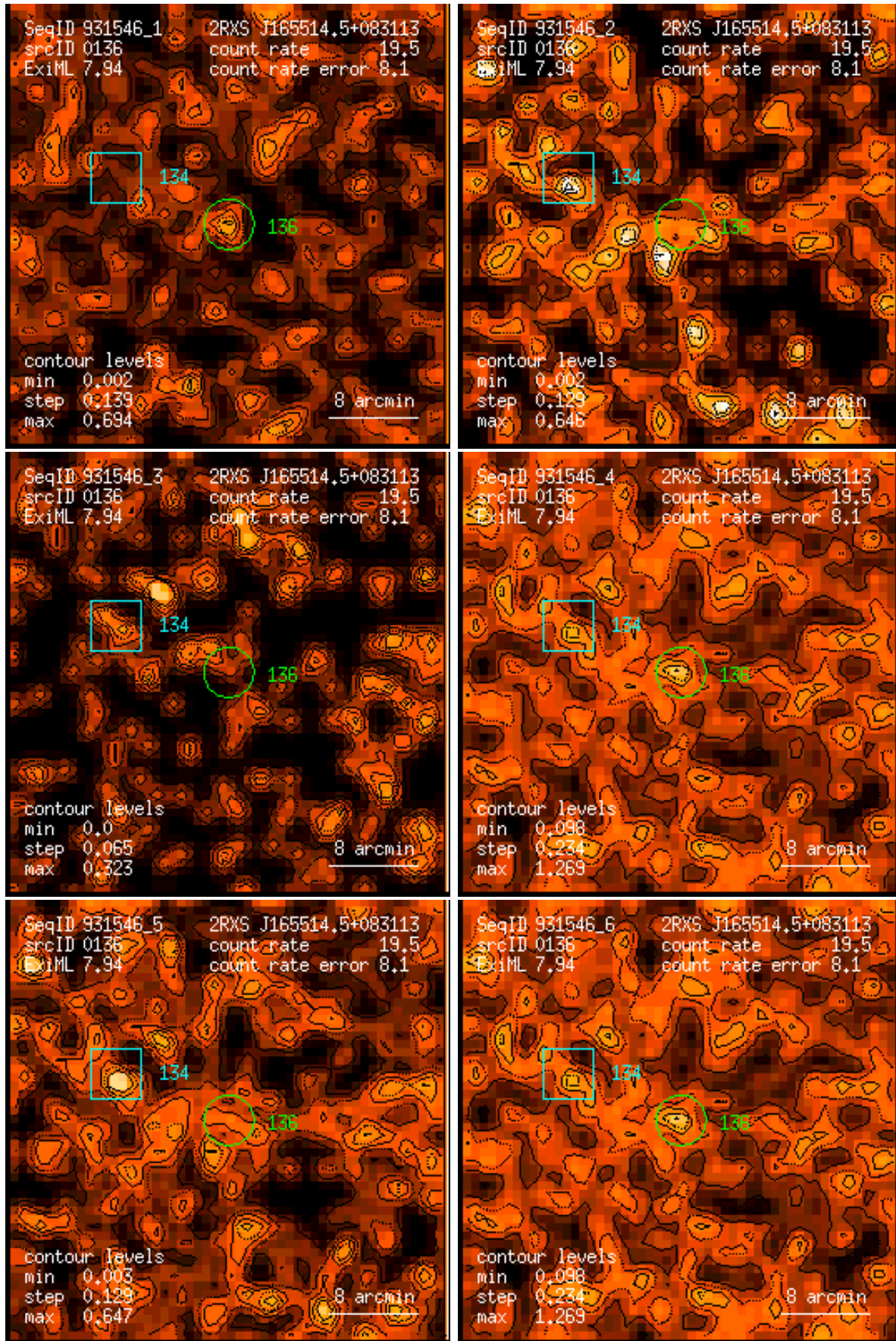
Figure 136: RASS 931546: detection 0136: band rate images, Gaussian filter: (1) PSPC channels 11 – 41, (2) 52 – 90, (3) 91 – 201, (4) 11 – 235, (5) 52 – 201, (6) 11 – 201. Broad band rates in counts/ks. Band rate contour levels in counts/ks/arcmin 2 .
